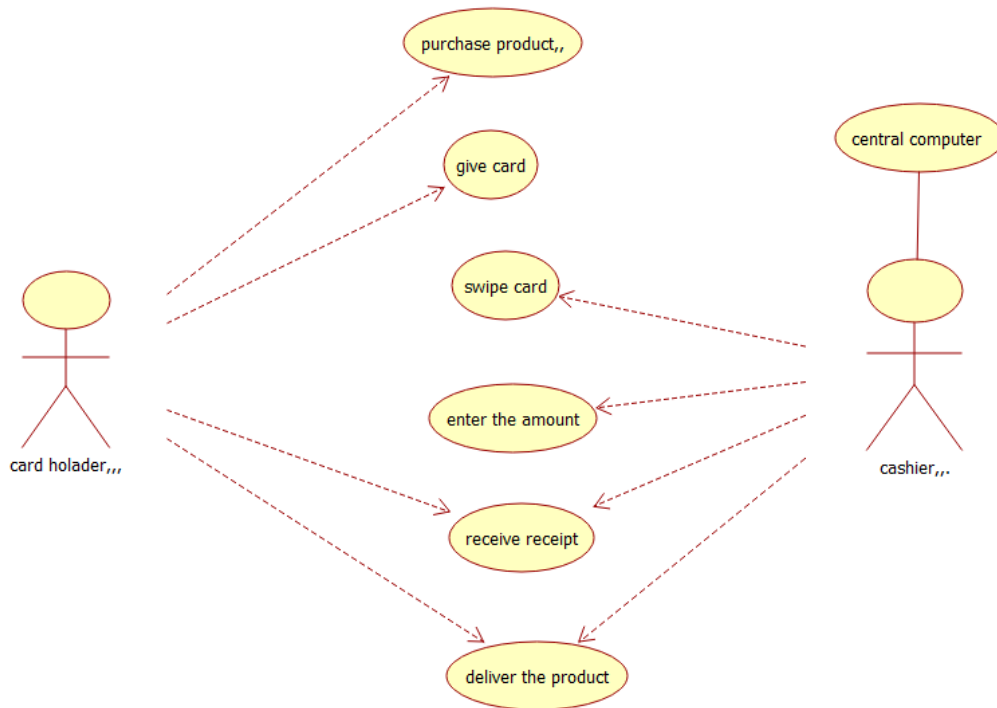
Diagram No: 1 Use Case Diagram
