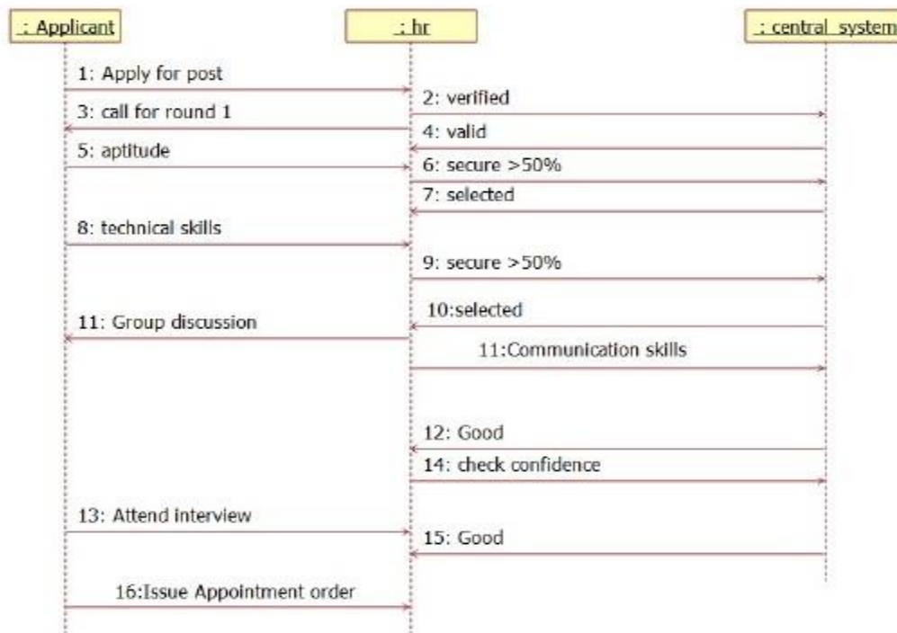
Diagram No: 4 Sequence Diagram
