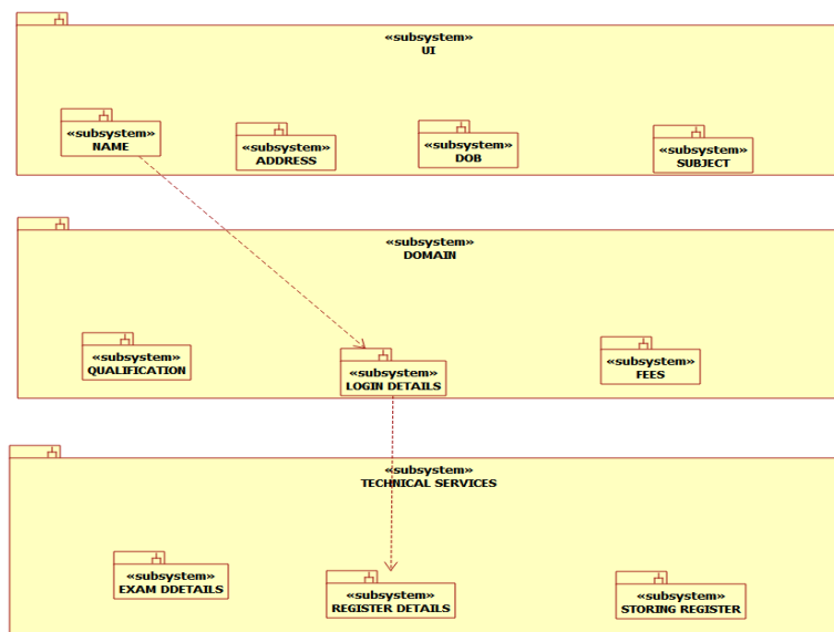
Diagram No: 9 Package Diagram
