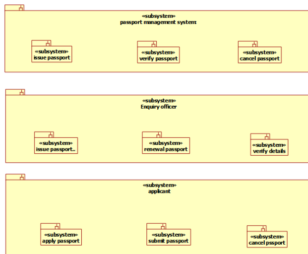
Diagram No: 9 Package Diagram
