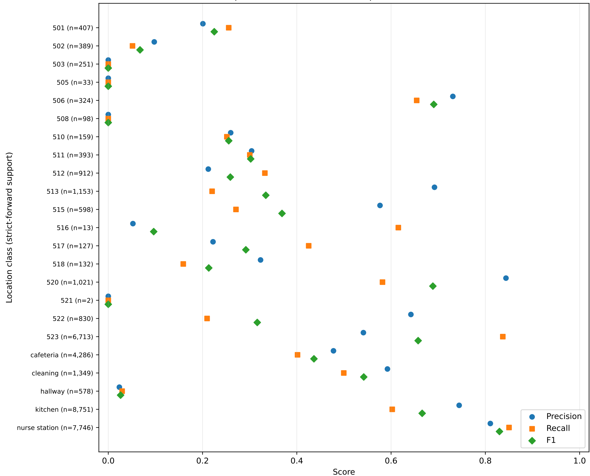
Final selected system: per-class classification metrics (pooled strict-forward development evaluation)
