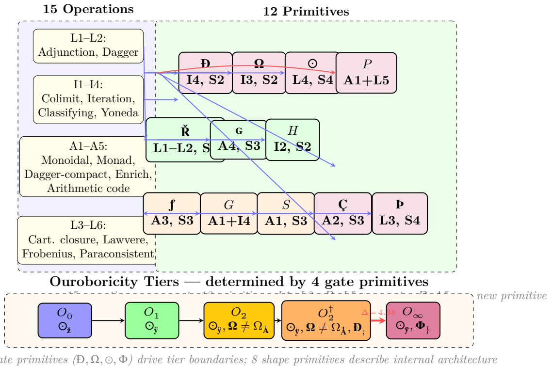
Figure 2: Complete mapping from 15 operations to 12 primitives. L1–L2 converge to \mathbf{\check{R}} ; A1 contributes to both \Sigma and \Phi ; L5 promotes \Phi (not a new primitive); A5 installs self-awareness without a new primitive. Bottom: ouroboricity tiers determined by the 4 gate primitives ( \mathbf{D}, \mathbf{\Omega}, \mathbf{\odot}, \mathbf{\Phi} ).
