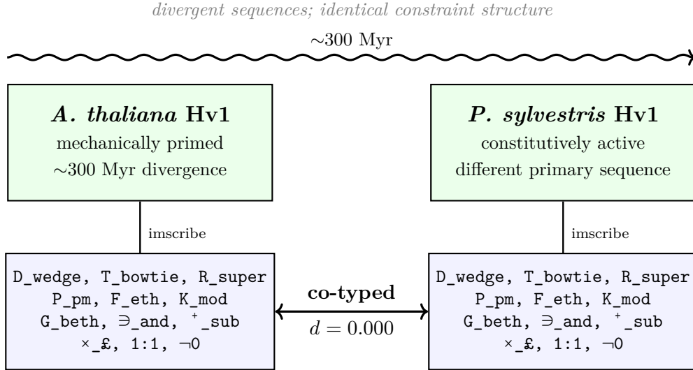
Figure 9: Hv1 proton channels: independent inscription convergence. Despite ~300 million years of evolutionary divergence, different primary sequences, and different regulatory mechanisms (mechanical priming vs. constitutive activity), A. thaliana and P. sylvestris Hv1 channels inscribe to identical 12-tuples ( d = 0.000 ). Both were inscribed independently using the twelve-step protocol. The convergence was neither designed nor expected.
