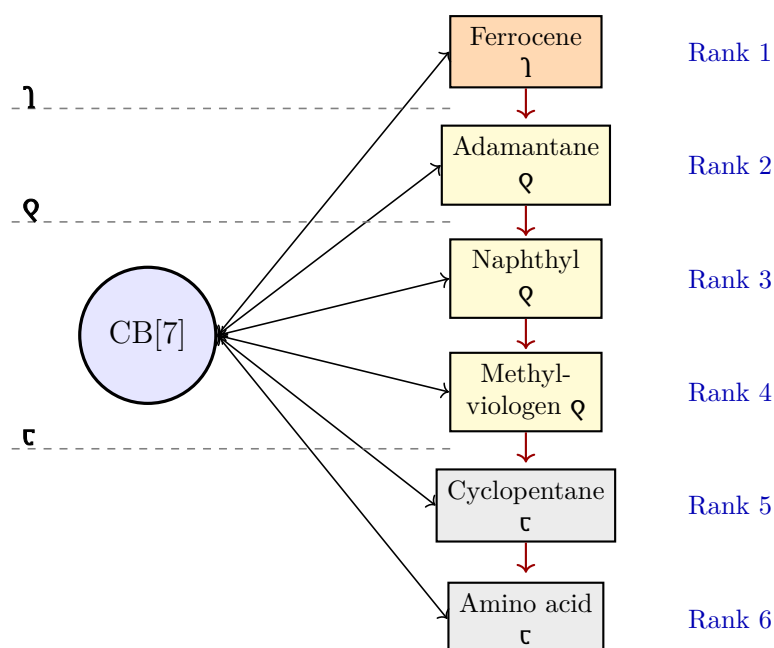
Figure 8: CB[7] competitive displacement predicted by the fidelity primitive. Guests are tiered by \equiv -ordinal ( \mathfrak{l} > \mathfrak{q} > \mathfrak{r} ). Within each \equiv -tier, finer structural distinctions determine rank. The grammar predicted the experimental order 6/6 using only this ordinal assignment, without binding-energy calculations or fitted parameters (Table 3).
