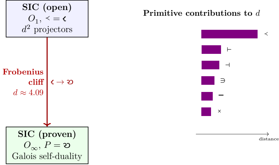
Figure 10: SIC-POVM Frobenius cliff . The open SIC conjecture occupies the O_1 tier with < = \zeta (approximate \mathbb{Z}_2 from pairwise equiangularity). The proven manifold occupies O_\infty with P = \psi (exact Frobenius self-duality). The gap d \approx 4.09 is dominated by the < -promotion ( \zeta \rightarrow \psi ), which cannot be closed by accumulation of dimension-by-dimension checks (Theorem 3). Galois descent from a Stark unit bypasses the cliff.
