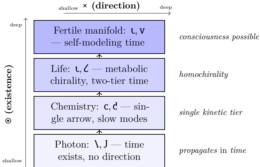
Figure 16: Time as \odot - \times coupling. \odot encodes the existence condition for time (kinetic depth \geq 1 required); \times encodes the direction condition (chirality/temporal asymmetry). The photon ( \lambda, J ) is the floor: it propagates in time but has no chirality or arrow of its own. Each cosmological phase transition deepens the \odot - \times coupling. The fertile manifold condition for consciousness requires \odot_{\text{depth}} \geq 2 and \times \geq \zeta : at minimum two kinetic tiers and two reinforcing chirality axes.
