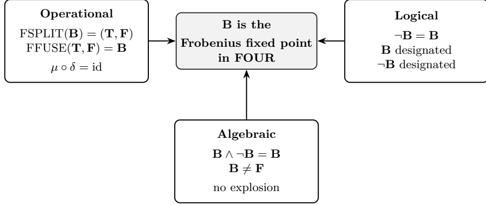
Figure 3: The Dialethic Alignment Theorem. Operational, logical, and algebraic perspectives on \mathbf{B} converge to a single structural fact: \mathbf{B} is the Frobenius fixed point in the Belnap lattice.
