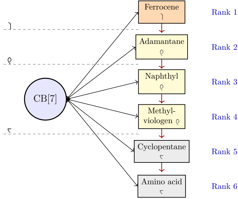
Figure 8: CB[7] competitive displacement predicted by the fidelity primitive. Guests are tiered by f-ordinal ( \lambda > \varrho > \tau ). Within each f-tier, finer structural distinctions determine rank. The grammar predicted the experimental order 6/6 using only this ordinal assignment, without binding-energy calculations or fitted parameters (Table 3).
