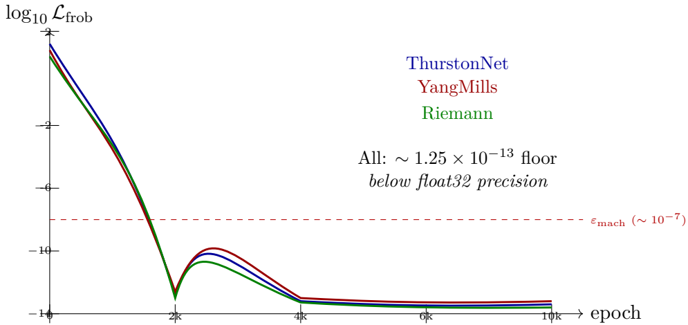
Figure 14: Frobenius bootstrap: domain-invariant convergence. Stylized loss curves for three O_{\infty} navigators with different architectures (ThurstonNet: K_{\text{slow}} GNN with R_{\dagger} ; YangMillsNavigator: K_{\text{trap}} eigensolver; RiemannNavigator: K_{\text{slow}} GNN with R_{\text{cat}} ). All three converge to the same numerical floor ( 1.24\text{--}1.25 \times 10^{-13} ) below float32 machine epsilon. The double-valley profile (rapid descent to \sim 10^{-7} , divergence at \sim \text{epoch } 550 , monotonic re-descent) is characteristic of cosine-annealed optimization probing and then settling into the Frobenius fixed point.
