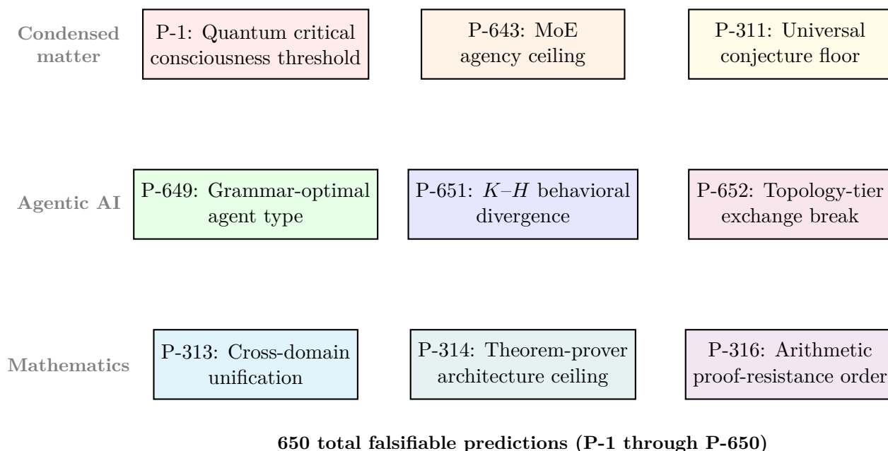
Figure 17: Selected predictions from the 650-entry registry. Predictions span condensed matter (P-1), agentic AI architecture (P-643, P-649), supramolecular chemistry (P-651, P-652), and pure mathematics (P-311, P-313, P-314, P-316). Each prediction is falsifiable from the inscribing protocol alone and carries a tier classification (Tier I: near-term empirical; Tier II: historical or architectural). The full registry is available in the supplementary catalog.
