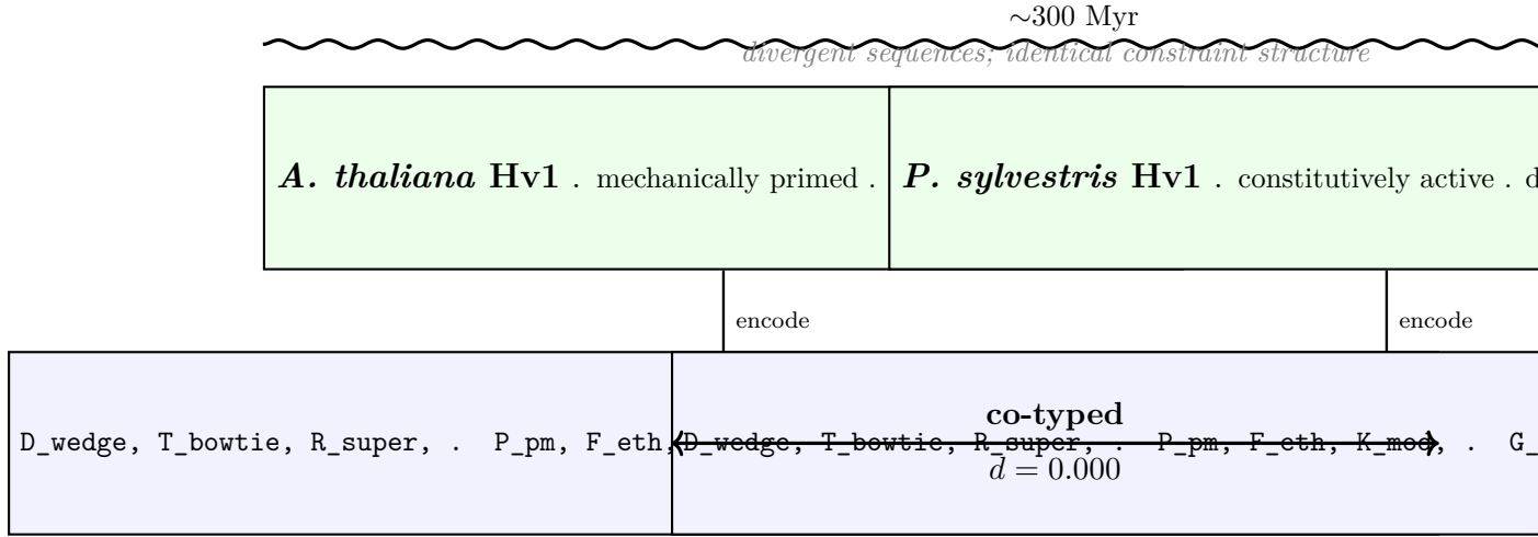
Figure 9: Hv1 proton channels: independent inscription convergence. Despite ~300 million years of evolutionary divergence, different primary sequences, and different regulatory mechanisms (mechanical priming vs. constitutive activity), A. thaliana and P. sylvestris Hv1 channels inscribe to identical 12-tuples ( d = 0.000 ). Both were inscribed independently using the twelve-step protocol. The convergence was neither designed nor expected.
