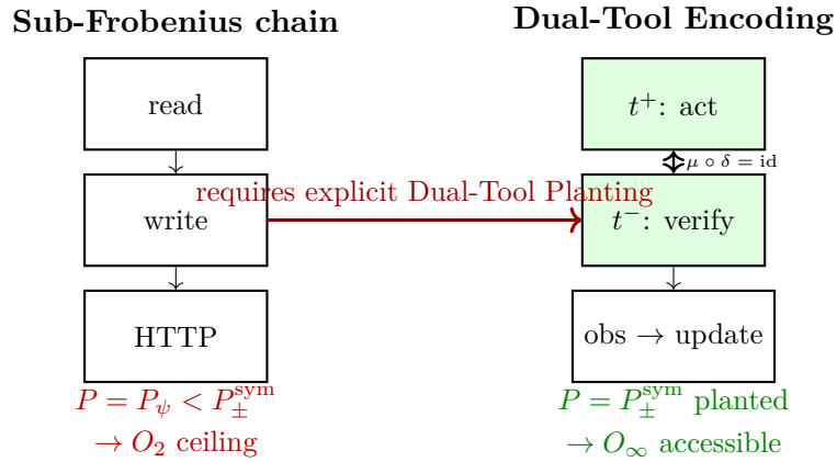
Figure 12: Dual-Tool Planting Theorem. Left: Standard tool calls have P = P_{\psi} < P_{\pm}^{\text{sym}} ; by Theorem 3, no sequence reaches O_{\infty} . Right: Pairing each tool call as (t^+, t^-) satisfying \mu \circ \delta(\text{query}) = \text{query} plants P_{\pm}^{\text{sym}} at the interface, making O_{\infty} structurally accessible. The grammar further predicts that deliberation loops without emission ( K_{\text{trap}} ) reduce C to 0, and that long-context agents undergo a D_{\Delta} \rightarrow D_{\odot} phase transition.
