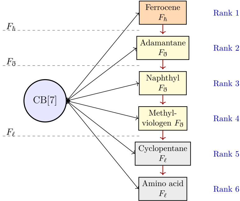
Figure 8: CB[7] competitive displacement predicted by the fidelity primitive. Guests are tiered by F -ordinal ( F_h > F_\delta > F_\ell ). Within each F -tier, finer structural distinctions determine rank. The grammar predicted the experimental order 6/6 using only this ordinal assignment, without binding-energy calculations or fitted parameters (Table 3).
