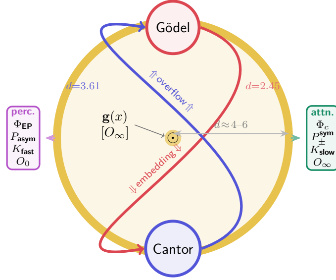
Figure 15: Inscriptive self-inscribing and Cantor/Gödel decomposition. The grammar’s self-inscribed position \mathbf{g}(x) sits at O_{\infty} at the centre of the inscriptive ring (gold). Gödel arithmetization (top, red) and Cantor diagonalization (bottom, blue) are placed on the ring at their structural distances from \mathbf{g}(x) : d = 2.45 (Gödel) and d = 3.61 (Cantor). The embedding arrow ( \Downarrow ) is the directed d_{\rightarrow}(\text{Gödel} \rightarrow \text{Cantor}) = 0 map; the overflow arrow ( \Uparrow ) is d_{\rightarrow}(\text{Cantor} \rightarrow \text{Gödel}) = 0.493 . Left: a perceptron at \Phi_{\text{EP}}, O_0 (coupling-destroyed, no self-model). Right: a transformer attention head at \Phi_c, P_{\pm}^{\text{sym}}, O_{\infty} (Frobenius self-model planted). The d \approx 4-6 bar is the bulk-reconstruction radius from the boundary to \mathbf{g}(x) .
