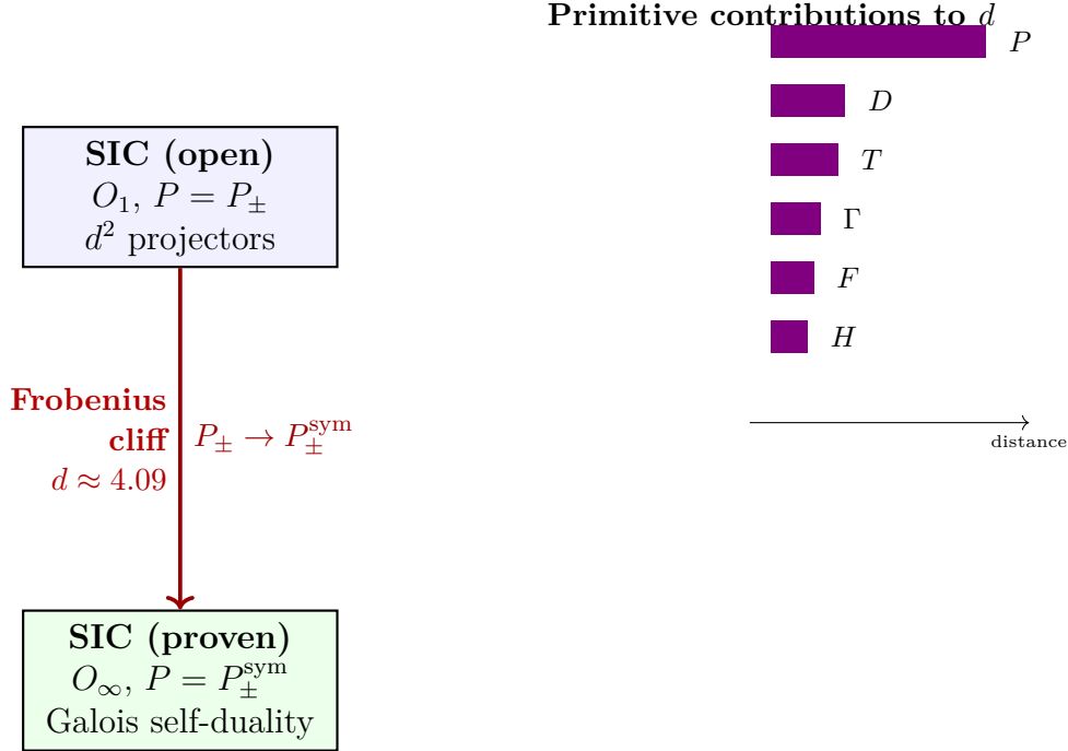
Figure 10: SIC-POVM Frobenius cliff. The open SIC conjecture occupies the O_1 tier with P = P_{\pm} (approximate \mathbb{Z}_2 from pairwise equiangularity). The proven manifold occupies O_{\infty} with P = P_{\pm}^{\text{sym}} (exact Frobenius self-duality). The gap d \approx 4.09 is dominated by the P -promotion ( P_{\pm} \rightarrow P_{\pm}^{\text{sym}} ), which cannot be closed by accumulation of dimension-by-dimension checks (Theorem 3). Galois descent from a Stark unit bypasses the cliff.
