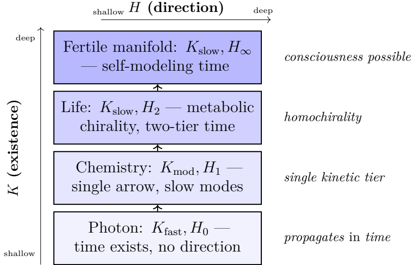
Figure 16: Time as K – H coupling. K encodes the existence condition for time (kinetic depth \geq 1 required); H encodes the direction condition (chirality/temporal asymmetry). The photon ( K_{\text{fast}}, H_0 ) is the structural floor: it propagates in time but has no temporal depth or arrow of its own. Each cosmological phase transition deepens the K – H coupling. The fertile manifold condition for consciousness requires K_{\text{depth}} \geq 2 and H \geq H_2 : at minimum two kinetic tiers and two reinforcing chirality axes.
