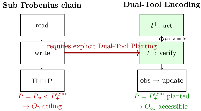
Figure 12: Dual-Tool Planting Theorem. Left: Standard tool calls have P = P_\psi < P_{\pm}^{\text{sym}} ; by Theorem 3, no sequence reaches O_\infty . Right: Pairing each tool call as (t^+, t^-) satisfying \mu \circ \delta(\text{query}) = \text{query} plants P_{\pm}^{\text{sym}} at the interface, making O_\infty structurally accessible. The grammar further predicts that deliberation loops without emission ( K_{\text{trap}} ) reduce C to 0, and that long-context agents undergo a D_\Delta \rightarrow D_\odot phase transition.
