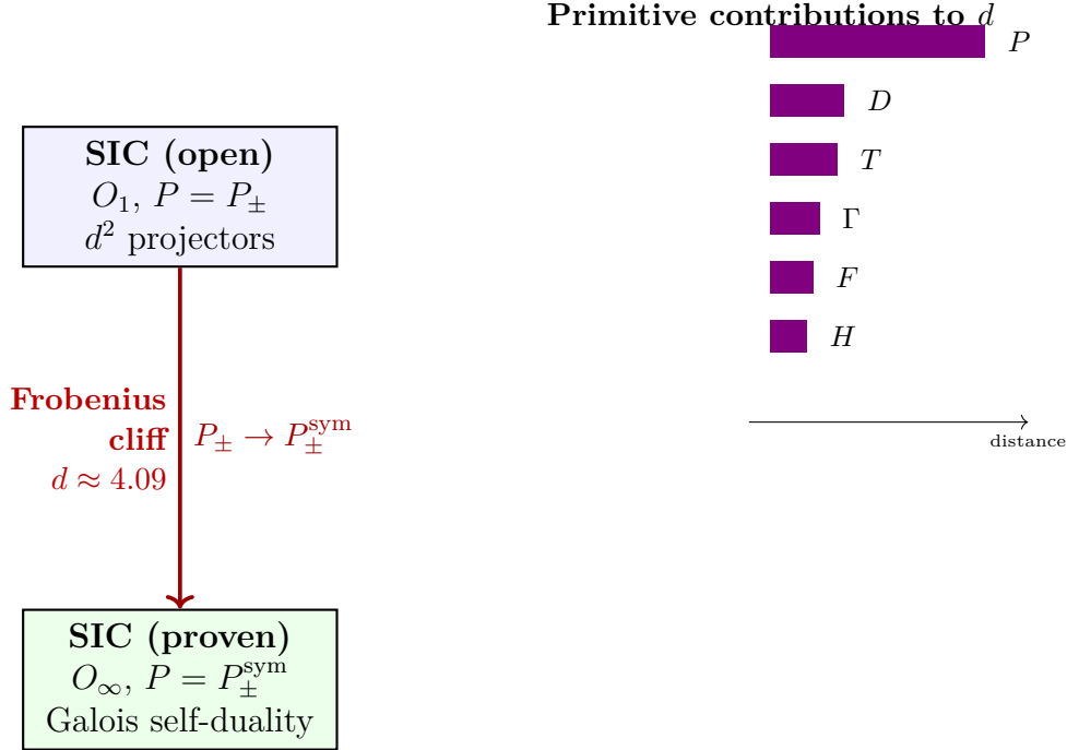
Figure 10: SIC-POVM Frobenius cliff. The open SIC conjecture occupies the O_1 tier with P = P_\pm (approximate \mathbb{Z}_2 from pairwise equiangularity). The proven manifold occupies O_\infty with P = P_\pm^{\text{sym}} (exact Frobenius self-duality). The gap d \approx 4.09 is dominated by the P -promotion ( P_\pm \rightarrow P_\pm^{\text{sym}} ), which cannot be closed by accumulation of dimension-by-dimension checks (Theorem 3). Galois descent from a Stark unit bypasses the cliff.
