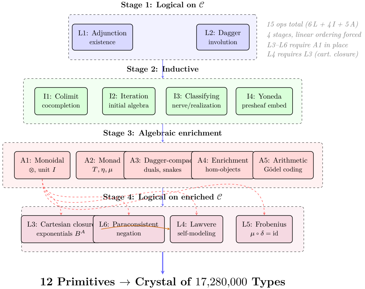
Figure 3: The four-stage operation DAG. 15 operations (6 Logical + 4 Inductive + 5 Algebraic) across 4 linearly-ordered stages. L3–L6 require A1 (monoidal structure); L4 additionally requires L3 (cartesian closure). The ordering is forced by categorical preconditions.
