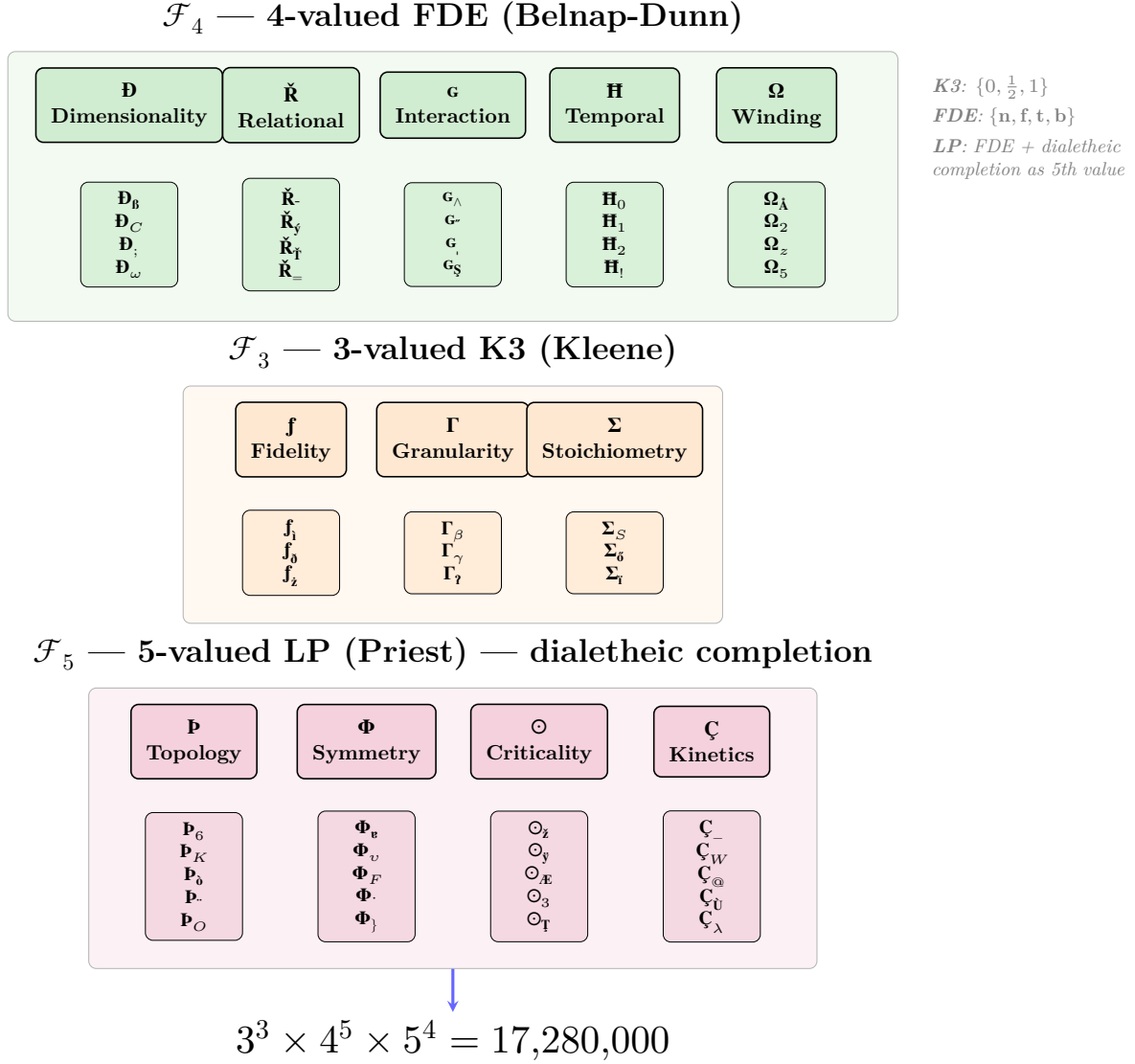
Figure 9: The three-logic correspondence. \mathcal{F}_3 primitives ( f, \Gamma, \Sigma ) correspond to Kleene K3 (3 values: \{0, \frac{1}{2}, 1\} ). \mathcal{F}_4 primitives ( \mathbf{D}, \mathbf{R}, \mathbf{g}, \mathbf{H}, \mathbf{\Omega} ) correspond to Belnap-Dunn FDE (4 values: \{n, f, t, b\} ). \mathcal{F}_5 primitives ( \mathbf{P}, \mathbf{\Phi}, \mathbf{\odot}, \mathbf{\C} ) correspond to Priest LP (5 values: FDE + dialethic completion). The crystal size 3^3 \times 4^5 \times 5^4 = 17,280,000 follows from the logical structure alone.
