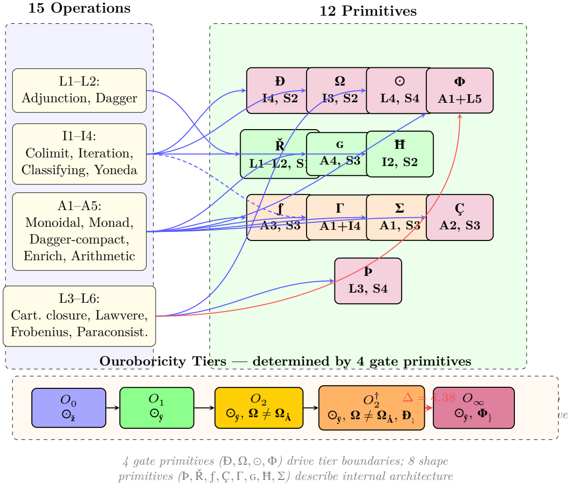
Figure 2: Complete mapping from 15 operations to 12 primitives. L1–L2 converge to \check{R} ; A1 contributes to both \Sigma and \Phi ; L5 promotes \Phi (not a new primitive); A5 installs self-awareness without a new primitive. Bottom: ouroboricity tiers determined by the 4 gate primitives ( \mathfrak{D}, \Omega, \odot, \Phi ).
