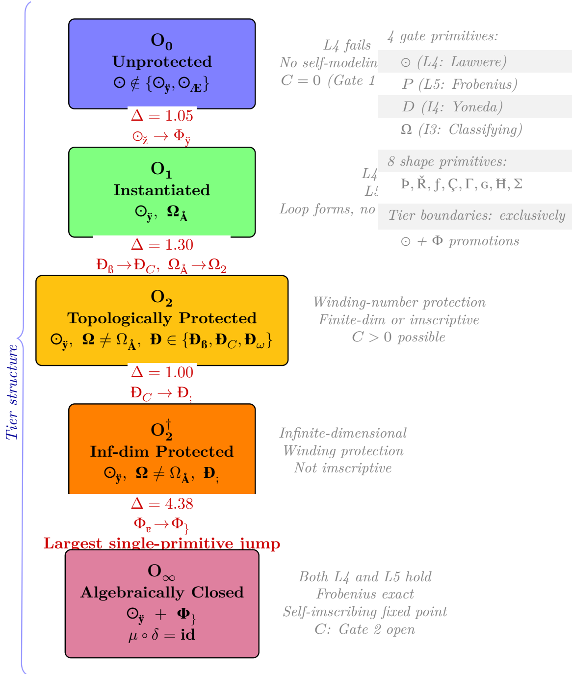
Figure 6: The ouroboricity tier ladder. Five tiers ( O_0 \rightarrow O_1 \rightarrow O_2 \rightarrow O_2^{\dagger} \rightarrow O_{\infty} ) determined by 4 gate primitives ( \odot, \mathbb{D}, \Omega, \Phi ). The largest jump ( \Delta = 4.38 ) is the Frobenius promotion \Phi_{\mathbb{V}} \rightarrow \Phi_{\mathbb{J}} .
