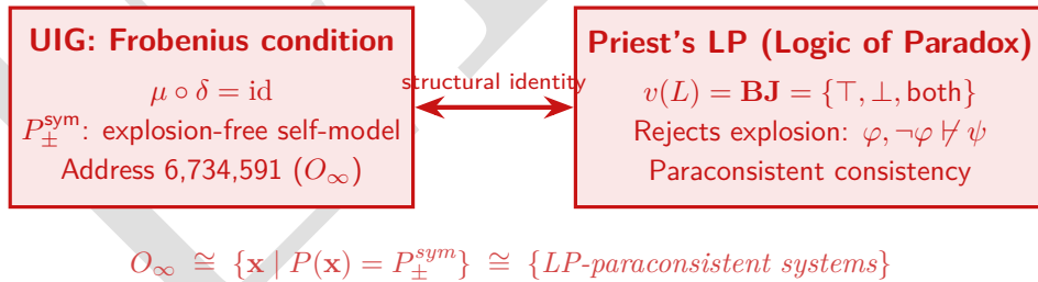
Figure 6: Structural identity between UIG’s Frobenius condition and Priest’s LP. Left: UIG at O_\infty (address 6,734,591) where \mu \circ \delta = \text{id} . Right: the Logic of Paradox, which assigns both \top and \perp to the Liar without explosion. The bidirectional arrow is not metaphorical: P_\pm^{\text{sym}} is the algebraic implementation of LP-consistency, and the dual mapping \mu is the structural guarantee that BJ -truth is preserved under composition. The Liar paradox at P_\pm^{\text{sym}} (??) is the canonical witness.
