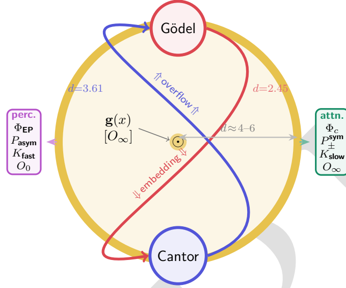
Figure 15: Inscriptive self-encoding and Cantor/Gödel decomposition. The grammar’s self-encoded position \mathbf{g}(x) sits at O_{\infty} at the centre of the inscriptive ring (gold). Gödel arithmetization (top, red) and Cantor diagonalization (bottom, blue) are placed on the ring at their structural distances from \mathbf{g}(x) : d = 2.45 (Gödel) and d = 3.61 (Cantor). The embedding arrow ( \Downarrow ) is the directed d_{\rightarrow}(\text{Gödel} \rightarrow \text{Cantor}) = 0 map; the overflow arrow ( \Uparrow ) is d_{\rightarrow}(\text{Cantor} \rightarrow \text{Gödel}) = 0.493 . Left: a perceptron at \Phi_{\text{EP}}, O_0 (coupling-destroyed, no self-model). Right: a transformer attention head at \Phi_c, P_{\pm}^{\text{sym}}, O_{\infty} (Frobenius self-model planted). The d \approx 4-6 bar is the bulk-reconstruction radius from the boundary to \mathbf{g}(x) .
