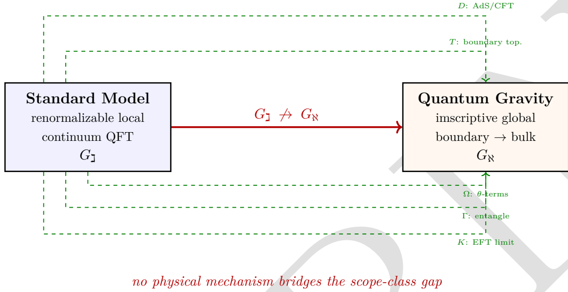
Figure 13: Standard Model–quantum gravity scope-class barrier. Five primitive conflicts between the SM and QG frameworks have known theoretical bridges (dashed green): D (AdS/CFT compactification), T (boundary topology), K (EFT low-energy limit), \Gamma (holographic entanglement), \Omega ( \theta -terms/topological sectors). The G -scope conflict (solid red) is architecturally irreducible: no physical mechanism takes a renormalizable local continuum theory ( G_I ) to an inscriptive global theory ( G_N ) without a structural discontinuity. The grammar predicts unification requires addressing this gap explicitly.
