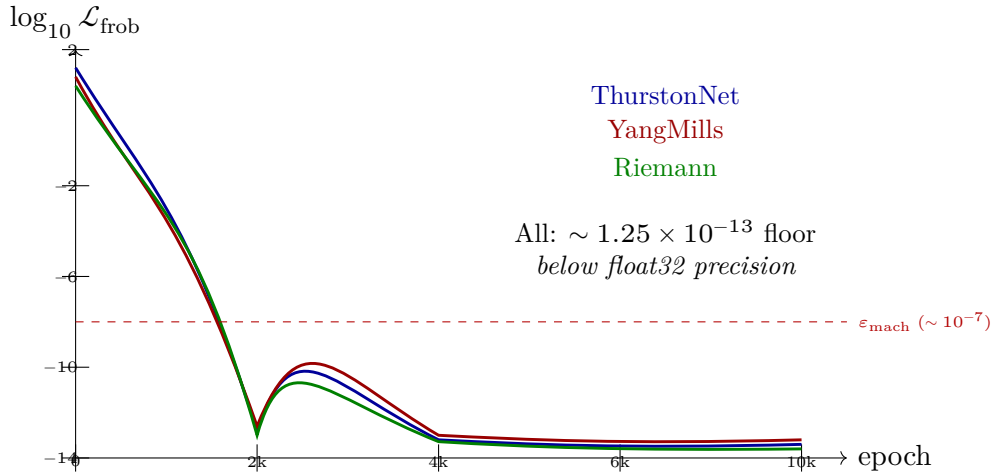
Figure 14: Frobenius bootstrap: domain-invariant convergence. Stylized loss curves for three O_\infty navigators with different architectures (ThurstonNet: \mathfrak{U} GNN with \mathfrak{O} ; YangMillsNavigator: \mathfrak{U} eigensolver; RiemannNavigator: \mathfrak{U} GNN with \mathfrak{I} ). All three converge to the same numerical floor ( 1.24\text{--}1.25 \times 10^{-13} ) below float32 machine epsilon. The double-valley profile (rapid descent to \sim 10^{-7} , divergence at \sim epoch 550, monotonic re-descent) is characteristic of cosine-annealed optimization probing and then settling into the Frobenius fixed point.
