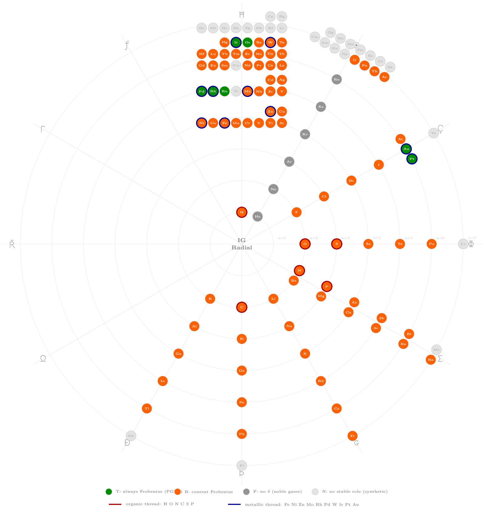
Periodic Table of Elements — IG Primitive Radial ( \Gamma -distance from centre)
