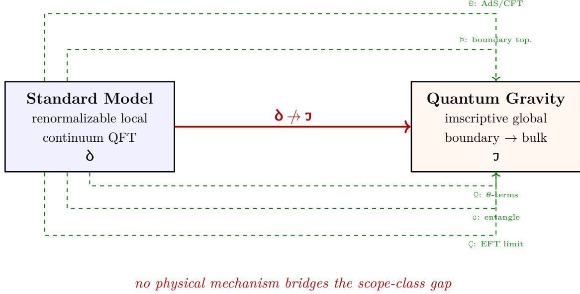
Figure 13: Standard Model–quantum gravity scope-class barrier. Five primitive conflicts between the SM and QG frameworks have known theoretical bridges (dashed green): \mathcal{D} (AdS/CFT compactification), \mathcal{P} (boundary topology), \mathcal{C} (EFT low-energy limit), \mathcal{G} (holographic entanglement), \mathcal{Q} ( \theta -terms/topological sectors). The \Gamma -scope conflict (solid red) is architecturally irreducible: no physical mechanism takes a renormalizable local continuum theory ( \delta ) to an imscriptive global theory ( \Gamma ) without a structural discontinuity. The grammar predicts unification requires addressing this gap explicitly.
