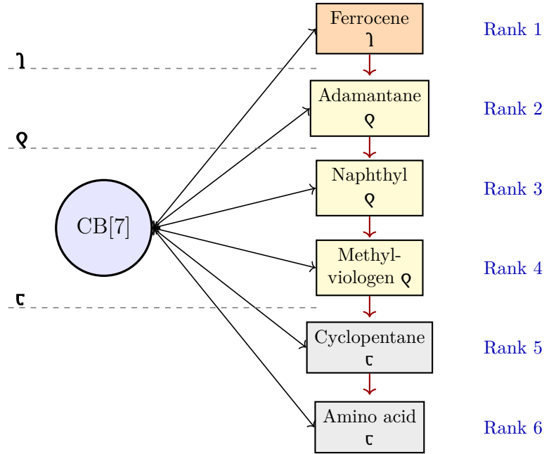
Figure 8: CB[7] competitive displacement predicted by the fidelity primitive. Guests are tiered by f -ordinal ( 1 > Q > \tau ). Within each f -tier, finer structural distinctions determine rank. The grammar predicted the experimental order 6/6 using only this ordinal assignment, without binding-energy calculations or fitted parameters (Table 3).
