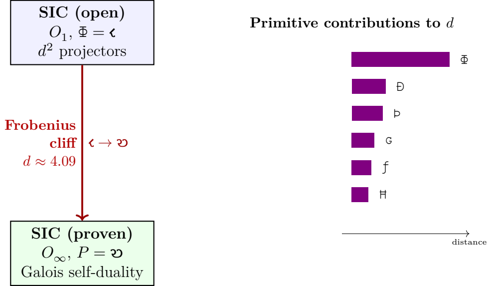
Figure 10: SIC-POVM Frobenius cliff. The open SIC conjecture occupies the O_1 tier with \Phi = \zeta (approximate \mathbb{Z}_2 from pairwise equiangularity). The proven manifold occupies O_\infty with P = \psi (exact Frobenius self-duality). The gap d \approx 4.09 is dominated by the \Phi -promotion ( \zeta \rightarrow \psi ), which cannot be closed by accumulation of dimension-by-dimension checks (Theorem 3). Galois descent from a Stark unit bypasses the cliff.
