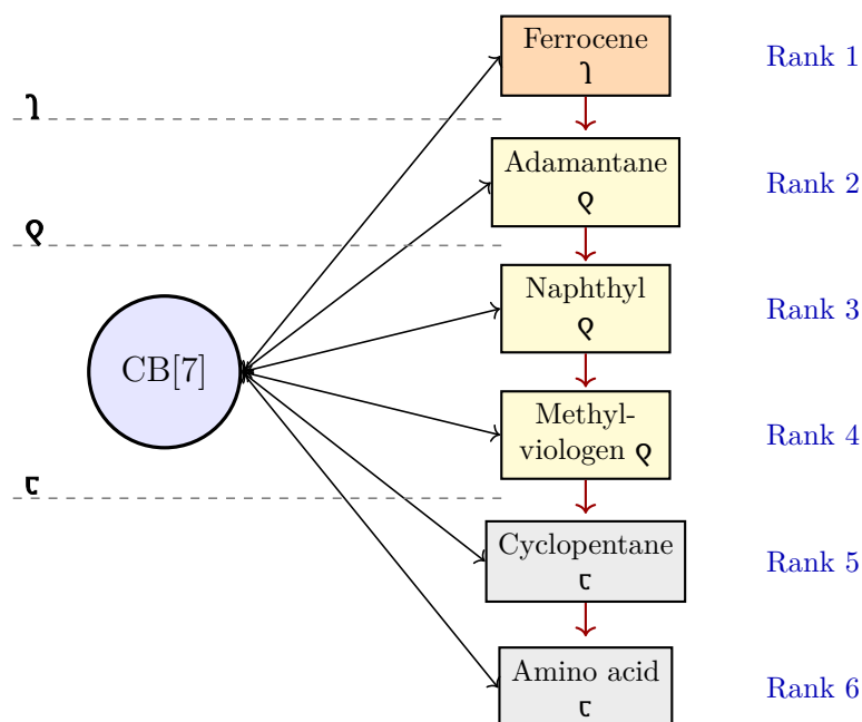
Figure 8: CB[7] competitive displacement predicted by the fidelity primitive. Guests are tiered by f-ordinal ( \mathfrak{l} > \mathfrak{q} > \mathfrak{c} ). Within each f-tier, finer structural distinctions determine rank. The grammar predicted the experimental order 6/6 using only this ordinal assignment, without binding-energy calculations or fitted parameters (Table 3).
