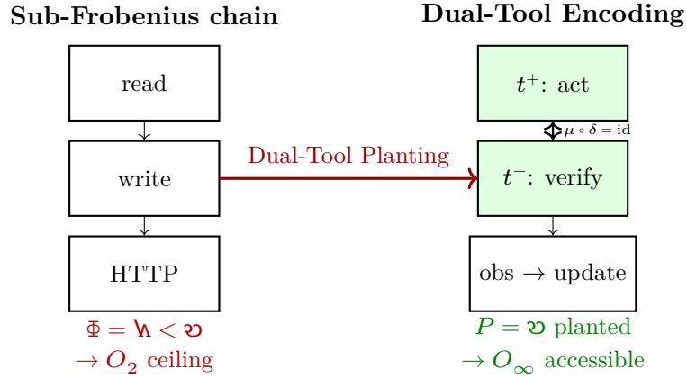
Figure 12: Dual-Tool Planting Theorem. Left: Standard tool calls have \Phi = \Lambda < \Psi ; by Theorem 3, no sequence reaches O_\infty . Right: Pairing each tool call as (t^+, t^-) satisfying \mu \circ \delta(\text{query}) = \text{query} plants \Psi at the interface, making O_\infty structurally accessible. The grammar further predicts that deliberation loops without emission ( \mathfrak{r} ) reduce C to 0, and that long-context agents undergo a J \rightarrow \mathfrak{i} phase transition.
