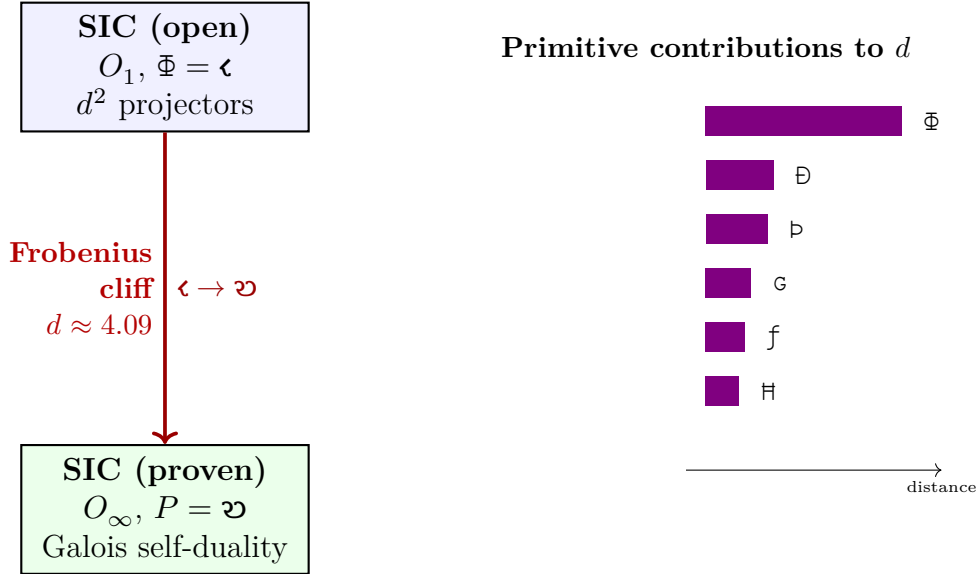
Figure 10: SIC-POVM Frobenius cliff . The open SIC conjecture occupies the O_1 tier with \Phi = \mathfrak{c} (approximate \mathbb{Z}_2 from pairwise equiangularity). The proven manifold occupies O_\infty with P = \mathfrak{v} (exact Frobenius self-duality). The gap d \approx 4.09 is dominated by the \Phi -promotion ( \mathfrak{c} \rightarrow \mathfrak{v} ), which cannot be closed by accumulation of dimension-by-dimension checks (Theorem 3). Galois descent from a Stark unit bypasses the cliff.
