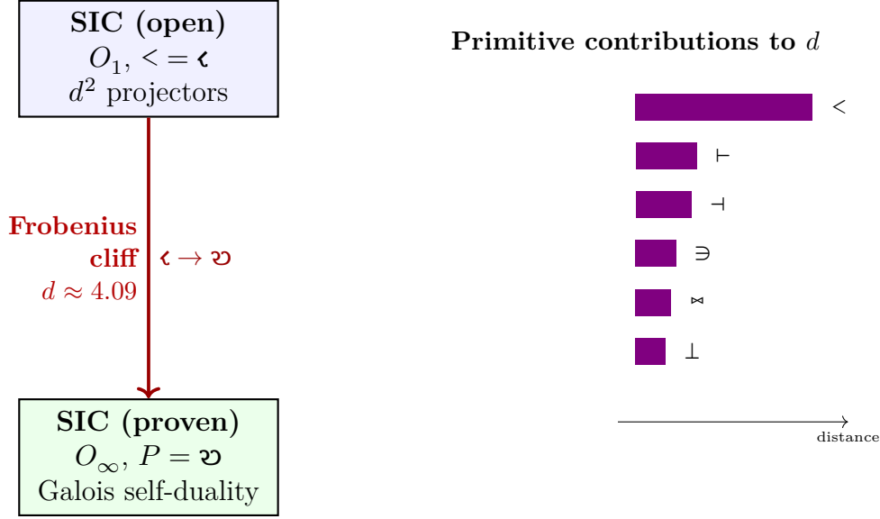
Figure 10: SIC-POVM Frobenius cliff . The open SIC conjecture occupies the O_1 tier with < = \swarrow (approximate \mathbb{Z}_2 from pairwise equiangularity). The proven manifold occupies O_\infty with P = \searrow (exact Frobenius self-duality). The gap d \approx 4.09 is dominated by the < -promotion ( \swarrow \rightarrow \searrow ), which cannot be closed by accumulation of dimension-by-dimension checks (Theorem 3). Galois descent from a Stark unit bypasses the cliff.
