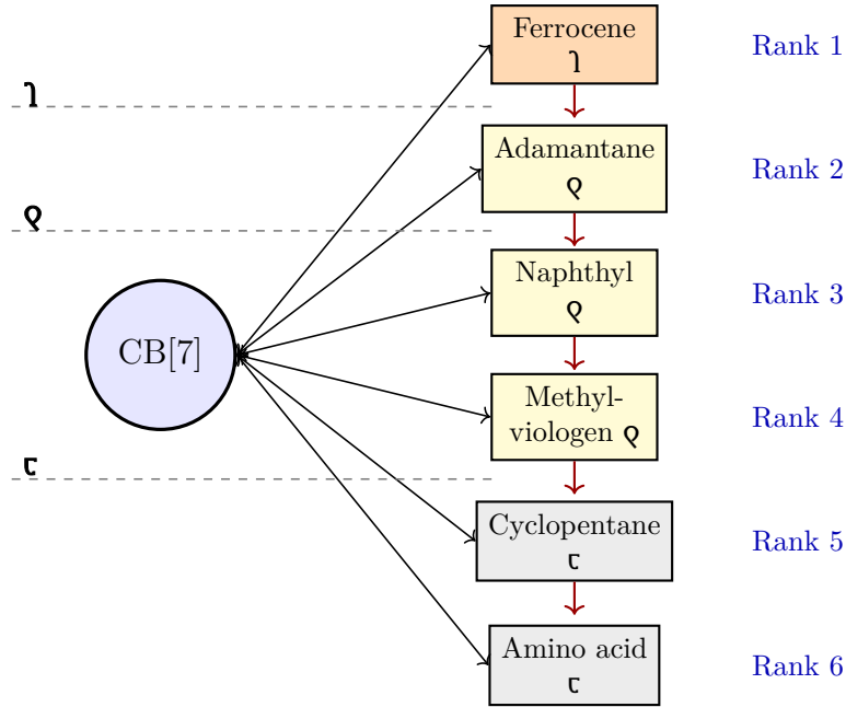
Figure 8: CB[7] competitive displacement predicted by the fidelity primitive. Guests are tiered by \preceq -ordinal ( 1 > 2 > 3 ). Within each \preceq -tier, finer structural distinctions determine rank. The grammar predicted the experimental order 6/6 using only this ordinal assignment, without binding-energy calculations or fitted parameters (Table 3).
