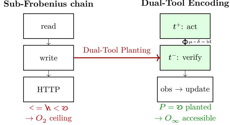
Figure 12: Dual-Tool Planting Theorem. Left: Standard tool calls have \leq \mathfrak{h} < \mathfrak{v} ; by Theorem 3, no sequence reaches O_\infty . Right: Pairing each tool call as (t^+, t^-) satisfying \mu \circ \delta(\text{query}) = \text{query} plants \mathfrak{v} at the interface, making O_\infty structurally accessible. The grammar further predicts that deliberation loops without emission ( \mathfrak{r} ) reduce C to 0, and that long-context agents undergo a \mathbf{J} \rightarrow \mathbf{1} phase transition.
