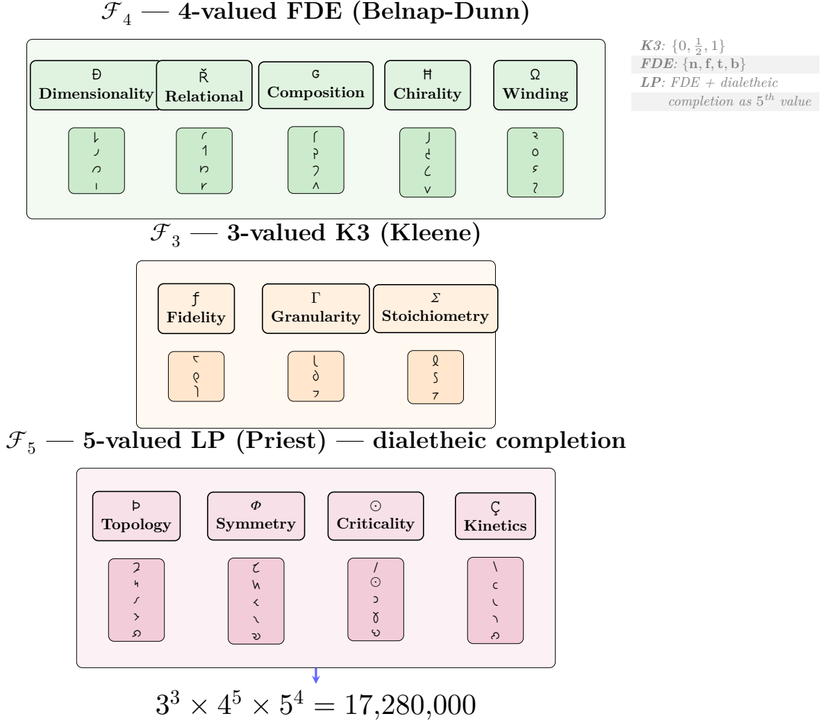
Figure 9: The three-logic correspondence. \mathcal{F}_3 primitives ( \mathfrak{f} , \Gamma , \Sigma ) correspond to Kleene K3 (3 values: \{0, \frac{1}{2}, 1\} ). \mathcal{F}_4 primitives ( \mathfrak{D} , \check{R} , \mathfrak{G} , \mathfrak{H} , \Omega ) correspond to Belnap-Dunn FDE (4 values: \{\mathbf{n}, \mathbf{f}, \mathbf{t}, \mathbf{b}\} ). \mathcal{F}_5 primitives ( \mathfrak{p} , \Phi , \odot , \mathfrak{C} ) correspond to Priest LP (5 values: FDE + dialethic completion). The crystal size 3^3 \times 4^5 \times 5^4 = 17,280,000 follows from the logical structure alone.
