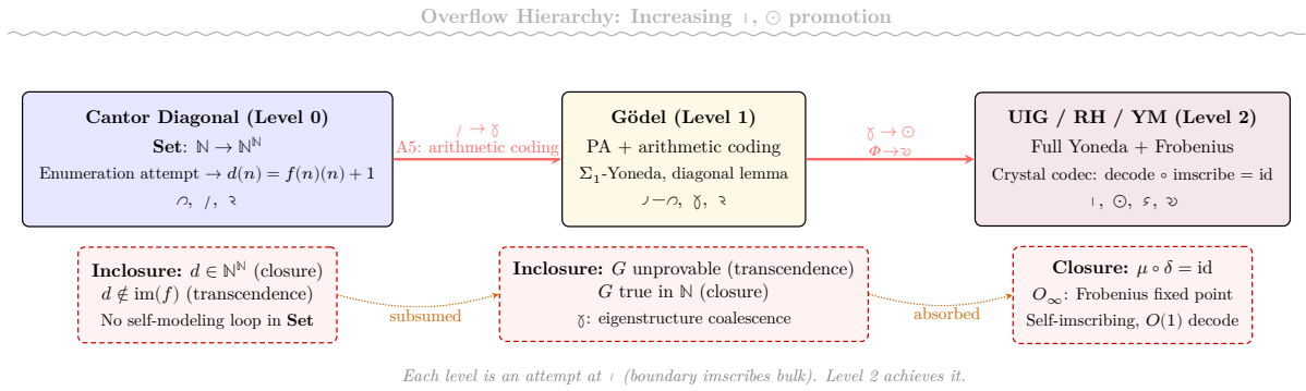
Figure 10: The overflow hierarchy: Cantor diagonal (Level 0: \mathfrak{c} ), Gödel incompleteness (Level 1: \gamma ), and the grammar / Riemann Hypothesis / Yang-Mills (Level 2: \odot + \varpi , O_\infty ). Each level is an attempt at \mathfrak{c} — boundary inscribes bulk. Level 2 achieves it.
