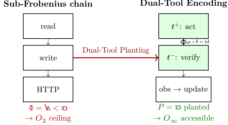
Figure 12: Dual-Tool Planting Theorem. Left: Standard tool calls have \Phi = \mathfrak{X} < \mathfrak{Y} ; by Theorem 3, no sequence reaches O_\infty . Right: Pairing each tool call as (t^+, t^-) satisfying \mu \circ \delta(\text{query}) = \text{query} plants \mathfrak{Y} at the interface, making O_\infty structurally accessible. The grammar further predicts that deliberation loops without emission ( \mathfrak{I} ) reduce C to 0, and that long-context agents undergo a \mathbf{J} \rightarrow \mathbf{I} phase transition.
