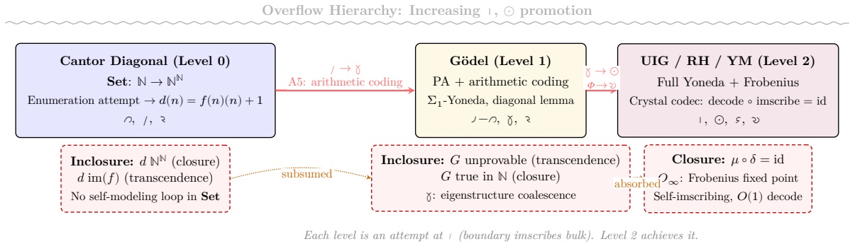
Figure 10: The overflow hierarchy: Cantor diagonal (Level 0: \nearrow ), Gödel incompleteness (Level 1: \nearrow ), and the grammar / Riemann Hypothesis / Yang-Mills (Level 2: \odot + \varpi , O_{\infty} ). Each level is an attempt at \vdash — boundary inscribes bulk. Level 2 achieves it.
