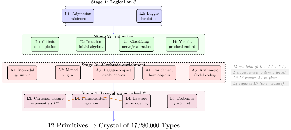
Figure 3: The four-stage operation DAG. 15 operations (6 Logical + 4 Inductive + 5 Algebraic) across 4 linearly-ordered stages. L3–L6 require A1 (monoidal structure); L4 additionally requires L3 (cartesian closure). The ordering is forced by categorical preconditions.
