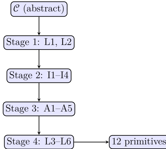
Figure 3: The four-stage operation DAG. 15 operations (6 Logical + 4 Inductive + 5 Algebraic) across 4 linearly-ordered stages. L3–L6 require A1 (monoidal structure); L4 additionally requires L3 (cartesian closure). The ordering is forced by categorical preconditions.
