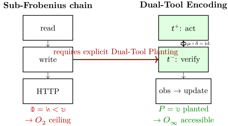
Figure 12: Dual-Tool Planting Theorem. Left: Standard tool calls have \Phi = \mathfrak{U} < \infty ; by Theorem 3, no sequence reaches O_\infty . Right: Pairing each tool call as (t^+, t^-) satisfying \mu \circ \delta(\text{query}) = \text{query} plants \infty at the interface, making O_\infty structurally accessible. The grammar further predicts that deliberation loops without emission ( \mathfrak{U} ) reduce C to 0, and that long-context agents undergo a \mathfrak{U} \rightarrow \mathfrak{I} phase transition.
