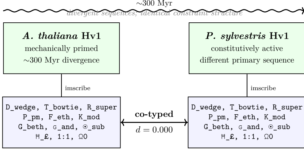
Figure 9: Hv1 proton channels: independent inscription convergence. Despite ~300 million years of evolutionary divergence, different primary sequences, and different regulatory mechanisms (mechanical priming vs. constitutive activity), A. thaliana and P. sylvestris Hv1 channels inscribe to identical 12-tuples ( d = 0.000 ). Both were inscribed independently using the twelve-step protocol. The convergence was neither designed nor expected.
