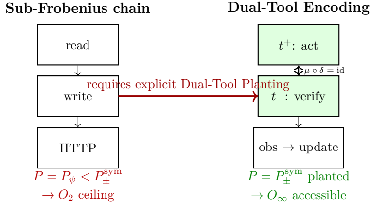
Figure 12: Dual-Tool Planting Theorem. Left: Standard tool calls have P = P_\psi < P_\pm^{\text{sym}} ; by Theorem 3, no sequence reaches O_\infty . Right: Pairing each tool call as (t^+, t^-) satisfying \mu \circ \delta(\text{query}) = \text{query} plants P_\pm^{\text{sym}} at the interface, making O_\infty structurally accessible. The grammar further predicts that deliberation loops without emission ( K_{\text{trap}} ) reduce C to 0, and that long-context agents undergo a D_\Delta \rightarrow D_\odot phase transition.
