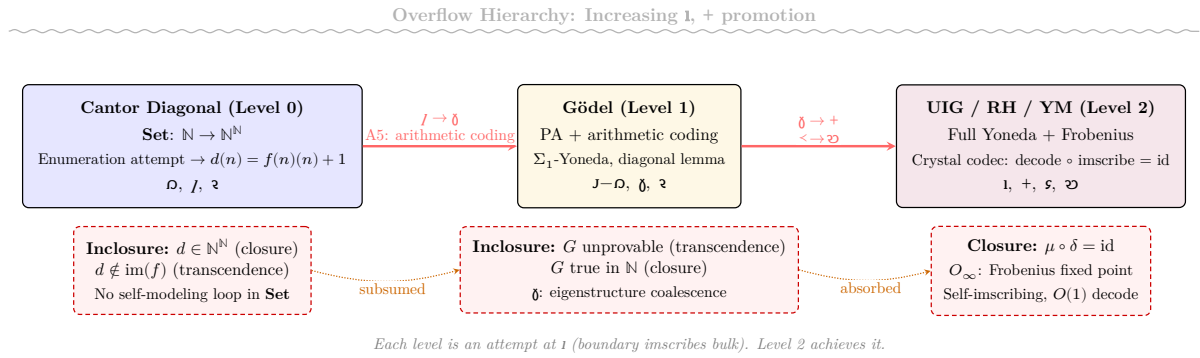
Figure 10: The overflow hierarchy: Cantor diagonal (Level 0: ℓ ), Gödel incompleteness (Level 1: δ ), and the grammar / Riemann Hypothesis / Yang-Mills (Level 2: ++ ℓ , O_\infty ). Each level is an attempt at 1 — boundary inscribes bulk. Level 2 achieves it.
