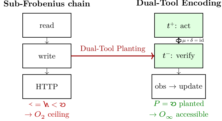
Figure 12: Dual-Tool Planting Theorem. Left: Standard tool calls have < = \mathfrak{A} < \mathfrak{B} ; by Theorem 3, no sequence reaches O_\infty . Right: Pairing each tool call as (t^+, t^-) satisfying \mu \circ \delta(\text{query}) = \text{query} plants \mathfrak{B} at the interface, making O_\infty structurally accessible. The grammar further predicts that deliberation loops without emission ( \mathfrak{A} ) reduce C to 0, and that long-context agents undergo a \mathbf{J} \rightarrow \mathbf{I} phase transition.
