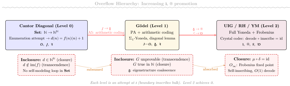
Figure 10: The overflow hierarchy: Cantor diagonal (Level 0: \mathfrak{I} ), Gödel incompleteness (Level 1: \mathfrak{d} ), and the grammar / Riemann Hypothesis / Yang-Mills (Level 2: \odot + \mathfrak{z} , O_{\infty} ). Each level is an attempt at 1 — boundary inscribes bulk. Level 2 achieves it.
