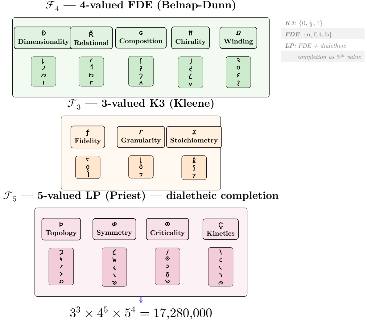
Figure 9: The three-logic correspondence. \mathcal{F}_3 primitives ( \mathfrak{f} , \mathfrak{r} , \mathfrak{s} ) correspond to Kleene K3 (3 values: \{0, \frac{1}{2}, 1\} ). \mathcal{F}_4 primitives ( \mathfrak{D} , \mathfrak{R} , \mathfrak{G} , \mathfrak{H} , \mathfrak{Q} ) correspond to Belnap-Dunn FDE (4 values: \{n, f, t, b\} ). \mathcal{F}_5 primitives ( \mathfrak{p} , \mathfrak{p} , \mathfrak{o} , \mathfrak{c} ) correspond to Priest LP (5 values: FDE + dialethic completion). The crystal size 3^3 \times 4^5 \times 5^4 = 17,280,000 follows from the logical structure alone.
