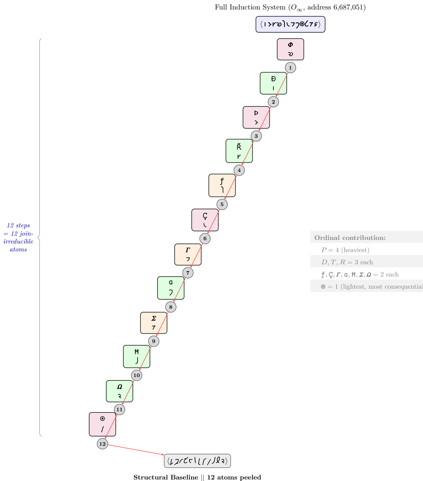
Figure 5: The 12-step retrosynthetic path from the full induction system ( O_\infty , address 6,687,051) to the structural baseline. Each step peels one primitive to its minimum value. Ordinal contributions: \Phi = 4 (heaviest), D, T, R = 3 each, f, \text{Ç}, \Gamma, G, H, \Sigma, \Omega = 2 each, \odot = 1 (lightest but most consequential for tier structure). All 12 steps are independent — no two primitives collapse together.
