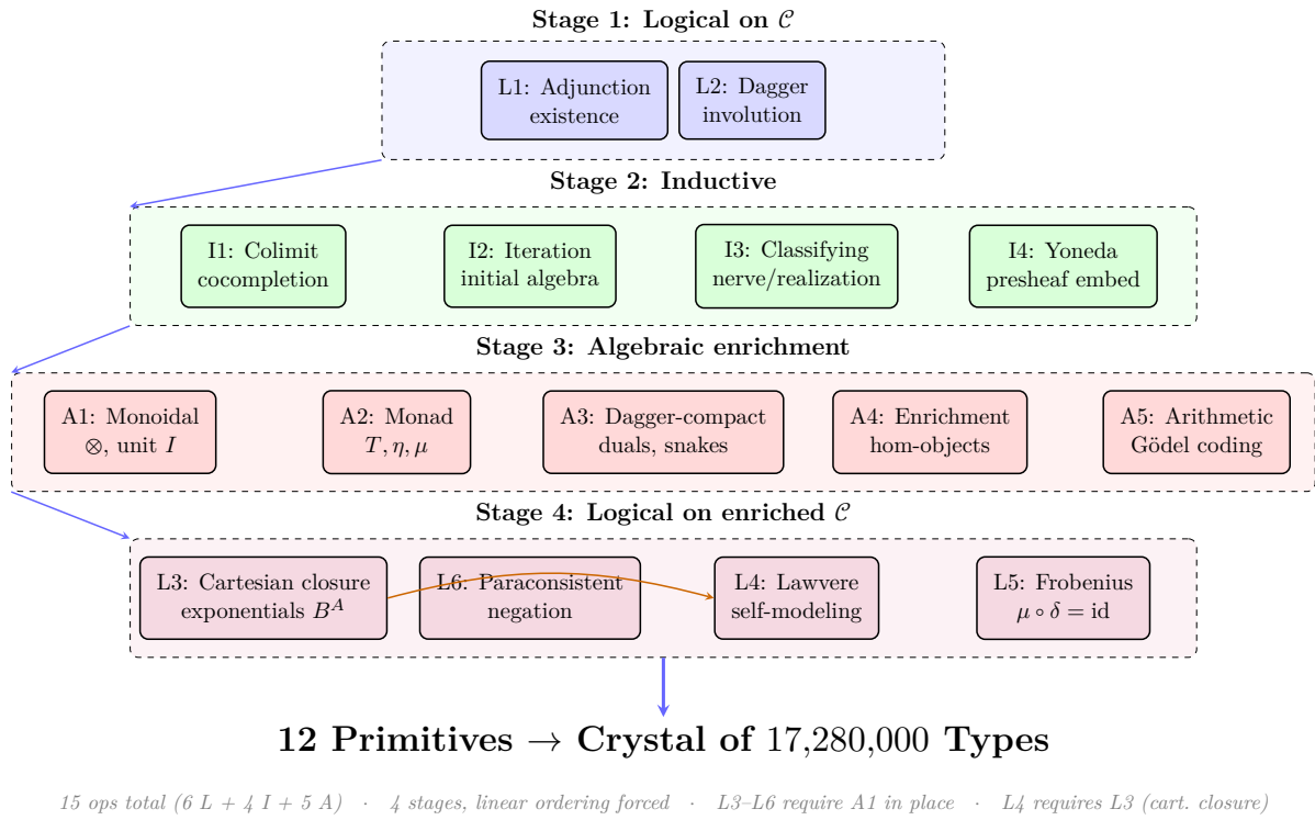
Figure 3: The four-stage operation DAG. 15 operations (6 Logical + 4 Inductive + 5 Algebraic) across 4 linearly-ordered stages. L3–L6 require A1 (monoidal structure); L4 additionally requires L3 (cartesian closure). The ordering is forced by categorical preconditions.
