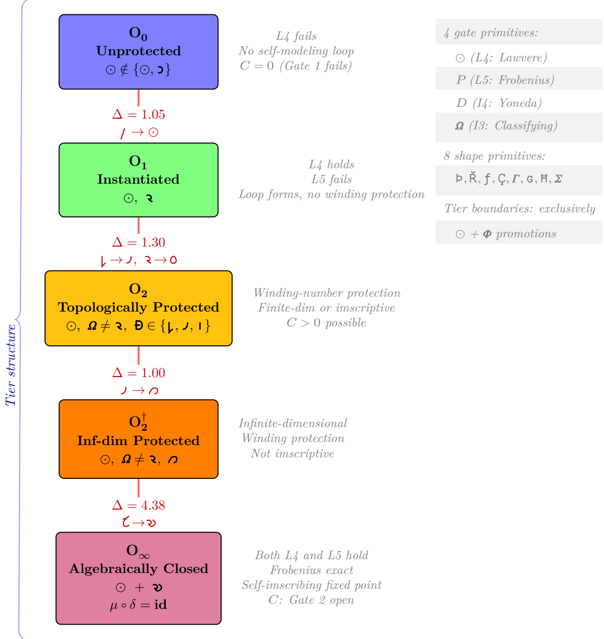
Figure 6: The ouroboricity tier ladder. Five tiers ( O_0 \rightarrow O_1 \rightarrow O_2 \rightarrow O_2^\dagger \rightarrow O_\infty ) determined by 4 gate primitives ( \odot, \mathfrak{D}, \mathfrak{Q}, \Phi ). The largest jump ( \Delta = 4.38 ) is the Frobenius promotion \mathfrak{Z} \rightarrow \mathfrak{V} .
