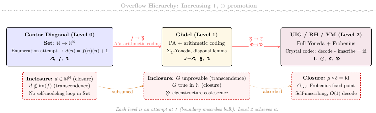
Figure 10: The overflow hierarchy: Cantor diagonal (Level 0: \mathbf{f} ), Gödel incompleteness (Level 1: \mathbf{J} ), and the grammar / Riemann Hypothesis / Yang-Mills (Level 2: \odot + \mathbf{v} , O_{\infty} ). Each level is an attempt at \mathbf{1} — boundary inscribes bulk. Level 2 achieves it.
