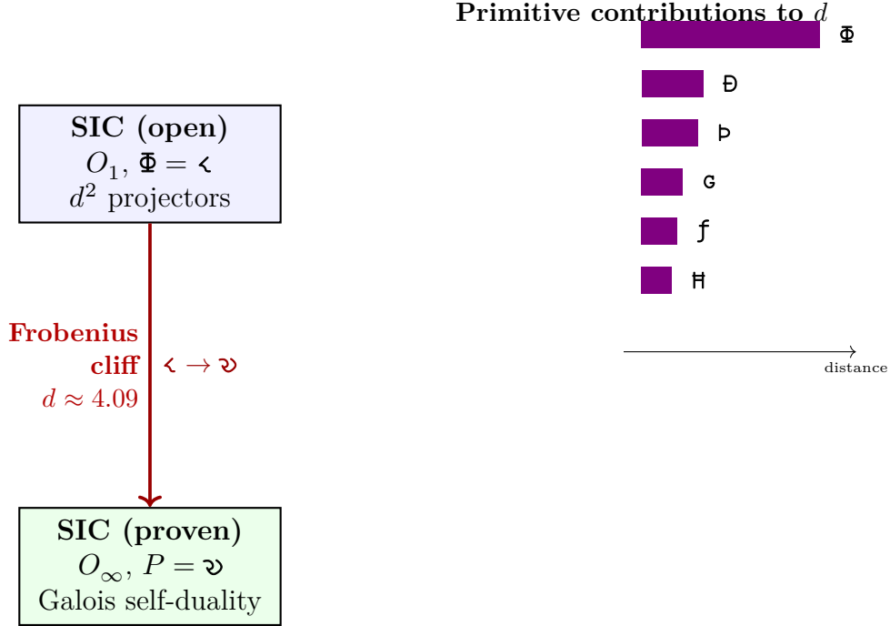
Figure 10: SIC-POVM Frobenius cliff . The open SIC conjecture occupies the O_1 tier with \Phi = \lhd (approximate \mathbb{Z}_2 from pairwise equiangularity). The proven manifold occupies O_\infty with P = \mathfrak{p} (exact Frobenius self-duality). The gap d \approx 4.09 is dominated by the \Phi -promotion ( \lhd \rightarrow \mathfrak{p} ), which cannot be closed by accumulation of dimension-by-dimension checks (Theorem 3). Galois descent from a Stark unit bypasses the cliff.
