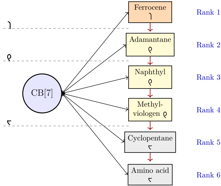
Figure 8: CB[7] competitive displacement predicted by the fidelity primitive. Guests are tiered by \mathbf{f} -ordinal ( \lambda > \rho > \tau ). Within each \mathbf{f} -tier, finer structural distinctions determine rank. The grammar predicted the experimental order 6/6 using only this ordinal assignment, without binding-energy calculations or fitted parameters (Table 3).
