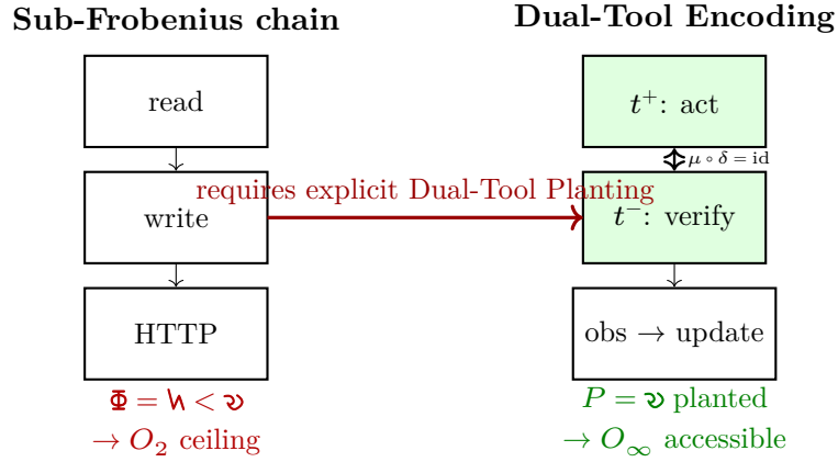
Figure 12: Dual-Tool Planting Theorem. Left: Standard tool calls have \Phi = \mathfrak{H} < \mathfrak{V} ; by Theorem 3, no sequence reaches O_\infty . Right: Pairing each tool call as (t^+, t^-) satisfying \mu \circ \delta(\text{query}) = \text{query} plants \mathfrak{V} at the interface, making O_\infty structurally accessible. The grammar further predicts that deliberation loops without emission ( \mathfrak{N} ) reduce C to 0, and that long-context agents undergo a \mathfrak{J} \rightarrow \mathfrak{I} phase transition.
