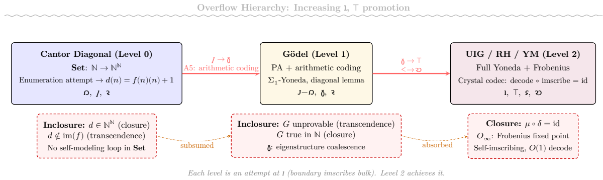
Figure 10: The overflow hierarchy: Cantor diagonal (Level 0: \mathfrak{I} ), Gödel incompleteness (Level 1: \delta ), and the grammar / Riemann Hypothesis / Yang-Mills (Level 2: \top + \mathfrak{V} , O_{\infty} ). Each level is an attempt at 1 — boundary inscribes bulk. Level 2 achieves it.
