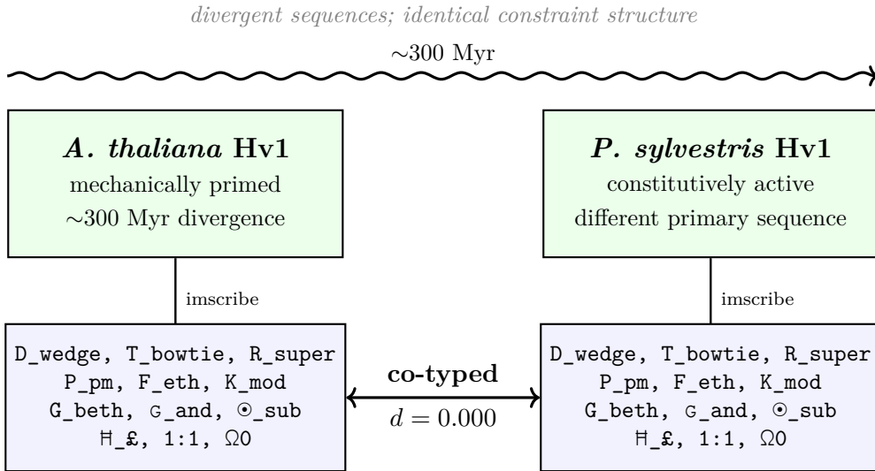
Figure 9: Hv1 proton channels: independent imscription convergence. Despite ~300 million years of evolutionary divergence, different primary sequences, and different regulatory mechanisms (mechanical priming vs. constitutive activity), A. thaliana and P. sylvestris Hv1 channels imscribe to identical 12-tuples ( d = 0.000 ). Both were imscribed independently using the twelve-step protocol. The convergence was neither designed nor expected.
