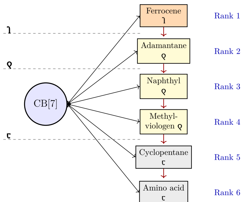
Figure 8: CB[7] competitive displacement predicted by the fidelity primitive. Guests are tiered by f -ordinal ( \mathfrak{l} > \mathfrak{q} > \mathfrak{c} ). Within each f -tier, finer structural distinctions determine rank. The grammar predicted the experimental order 6/6 using only this ordinal assignment, without binding-energy calculations or fitted parameters (Table 3).
