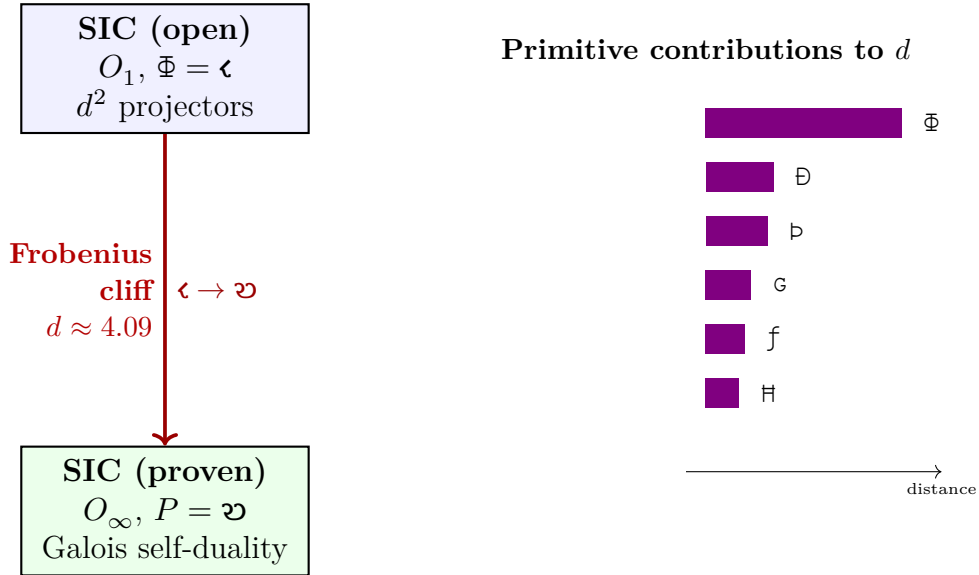
Figure 10: SIC-POVM Frobenius cliff . The open SIC conjecture occupies the O_1 tier with \Phi = \zeta (approximate \mathbb{Z}_2 from pairwise equiangularity). The proven manifold occupies O_\infty with P = \vartheta (exact Frobenius self-duality). The gap d \approx 4.09 is dominated by the \Phi -promotion ( \zeta \rightarrow \vartheta ), which cannot be closed by accumulation of dimension-by-dimension checks (Theorem 3). Galois descent from a Stark unit bypasses the cliff.
