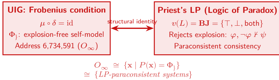
Figure 6: Structural identity between UIG's Frobenius condition and Priest's LP. Left: UIG at O_{\infty} (address 6,734,591) where \mu \circ \delta = \text{id} . Right: the Logic of Paradox, which assigns both \top and \perp to the Liar without explosion. The bidirectional arrow is not metaphorical: \Phi_{\downarrow} is the algebraic implementation of LP-consistency, and the dual mapping \mu is the structural guarantee that BJ -truth is preserved under composition. The Liar paradox at \Phi_{\downarrow} (Equation (11)) is the canonical witness.
