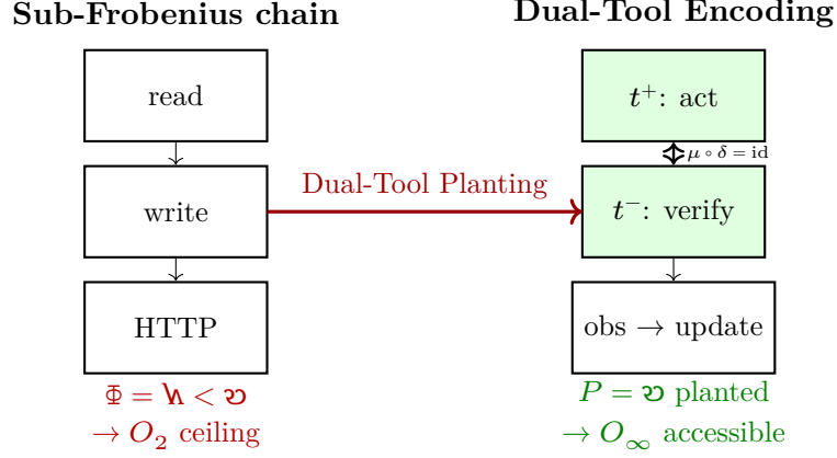
Figure 12: Dual-Tool Planting Theorem. Left: Standard tool calls have \Phi = \mathbf{1} < \mathbf{2} ; by Theorem 3, no sequence reaches O_\infty . Right: Pairing each tool call as (t^+, t^-) satisfying \mu \circ \delta(\text{query}) = \text{query} plants \mathbf{2} at the interface, making O_\infty structurally accessible. The grammar further predicts that deliberation loops without emission ( \mathbf{1} ) reduce C to 0, and that long-context agents undergo a \mathbf{J} \rightarrow \mathbf{1} phase transition.
