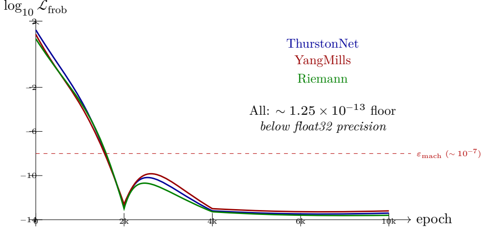
Figure 14: Frobenius bootstrap: domain-invariant convergence. Stylized loss curves for three O_\infty navigators with different architectures (ThurstonNet: \mathfrak{t} GNN with \mathfrak{n} ; YangMillsNavigator: \mathfrak{r} eigensolver; RiemannNavigator: \mathfrak{t} GNN with \mathfrak{1} ). All three converge to the same numerical floor ( 1.24\text{--}1.25 \times 10^{-13} ) below float32 machine epsilon. The double-valley profile (rapid descent to \sim 10^{-7} , divergence at \sim epoch 550, monotonic re-descent) is characteristic of cosine-annealed optimization probing and then settling into the Frobenius fixed point.
