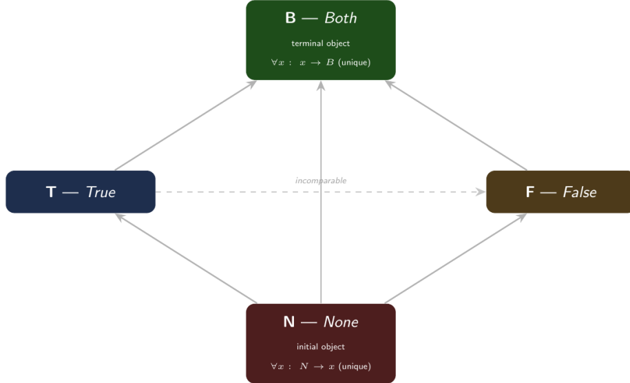
Figure 7: The Belnap lattice as a category. N is the unique initial object (unique arrow to everything). B is the unique terminal object (unique arrow from everything). The terminal object is also the Frobenius fixed point — a coincidence that is not general categorical fact but specific to B , and the reason the kernel can sustain indefinite paradox.
