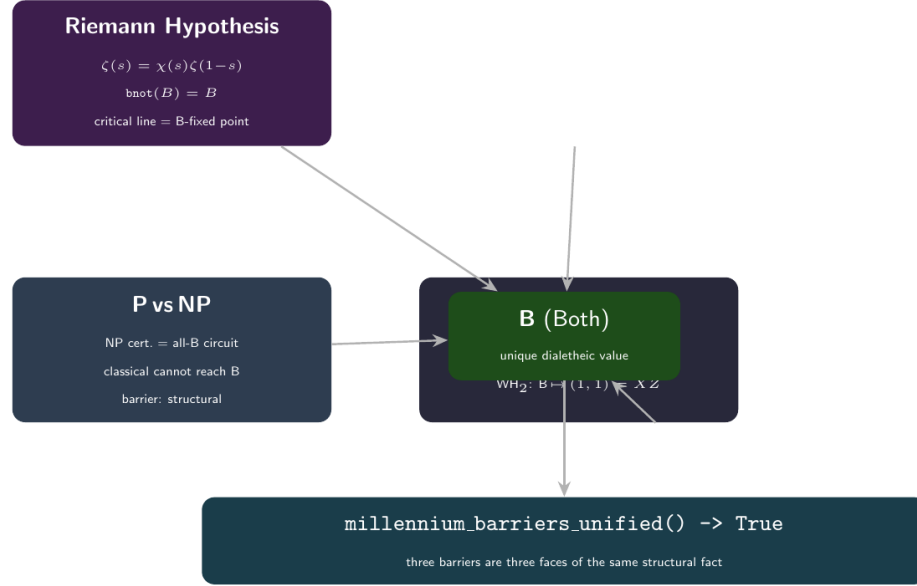
Figure 5: Four Millennium Problems converging on the same structural bottleneck. B is not a solution to any of them — it is the point where their structural formulations coincide. The Riemann Hypothesis becomes a fixed point of negation; the Yang-Mills mass gap becomes a covering relation in the Belnap approximation order; P vs NP becomes a one-way barrier from classical to paraconsistent circuits; SIC-POVM becomes the self-adjoint structure of B .
