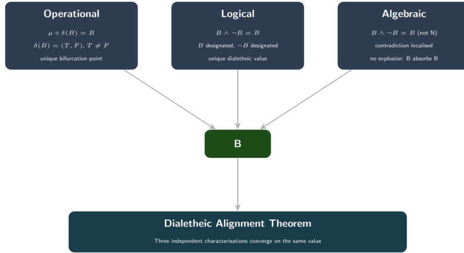
Figure 4: The Dialethic Alignment Theorem — three independent characterizations of B (operational, logical, algebraic) converge on the same value. The theorem is not deep (it follows from the Belnap lattice definition) but its consequences cascade through Millennium Problem structure.
