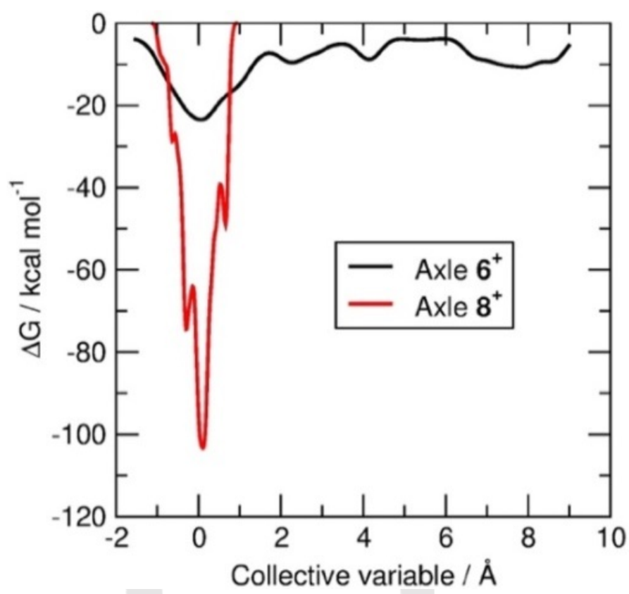
Figure 2: Schematic free-energy profiles for DB24C8 dethreading
