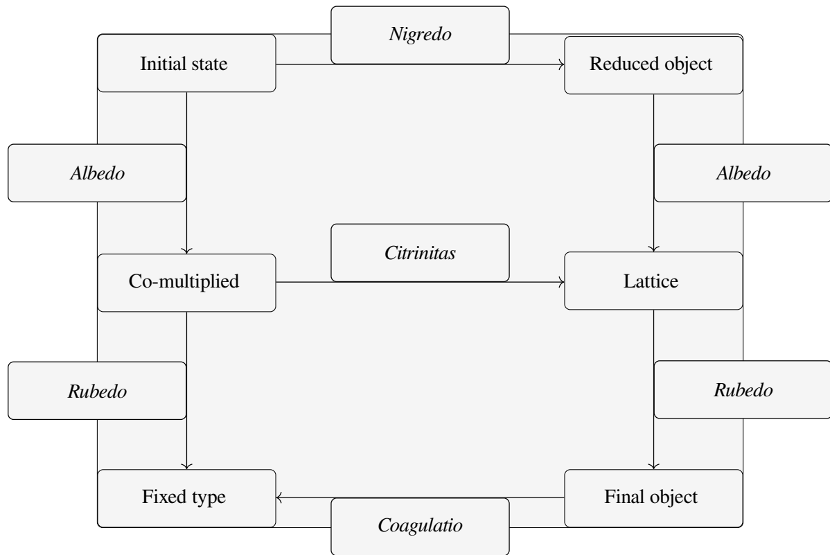
Figure 1: The alchemical commutative square. The four classical stages label the morphisms of the Frobenius bialgebra. Albedo ( \text{FSPLIT}/\delta ) appears on both sides as a natural transformation applied uniformly, not two distinct operations. Coagulatio ( \text{FFUSE}/\mu , bottom arrow) closes the Frobenius pair; without it the square has an open split—the biological section’s failure mode. The primary path is the right column: Initial \xrightarrow{\text{Nigredo}} Reduced \xrightarrow{\text{Albedo}} Lattice \xrightarrow{\text{Rubedo}} Final object.
