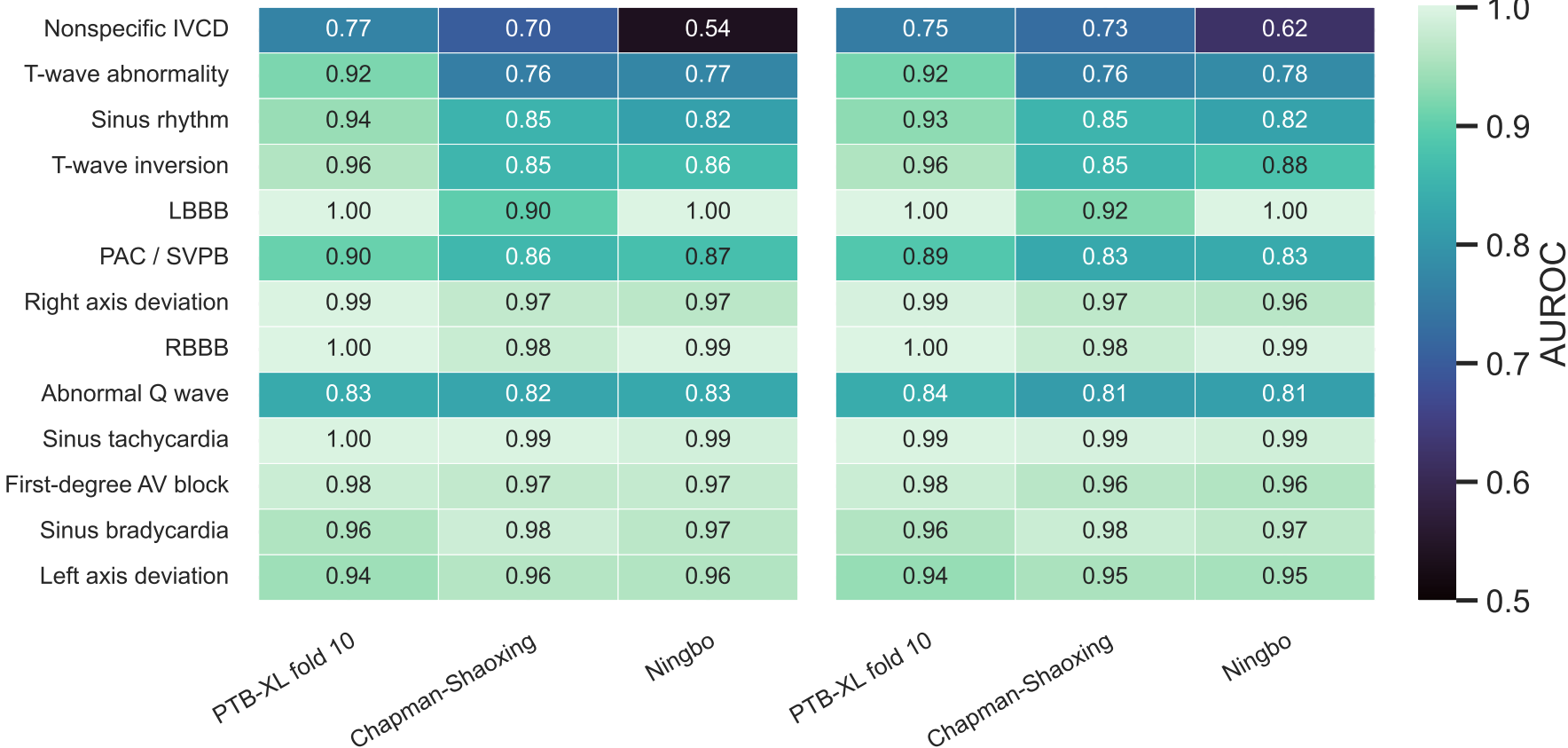
xResNet1d101
