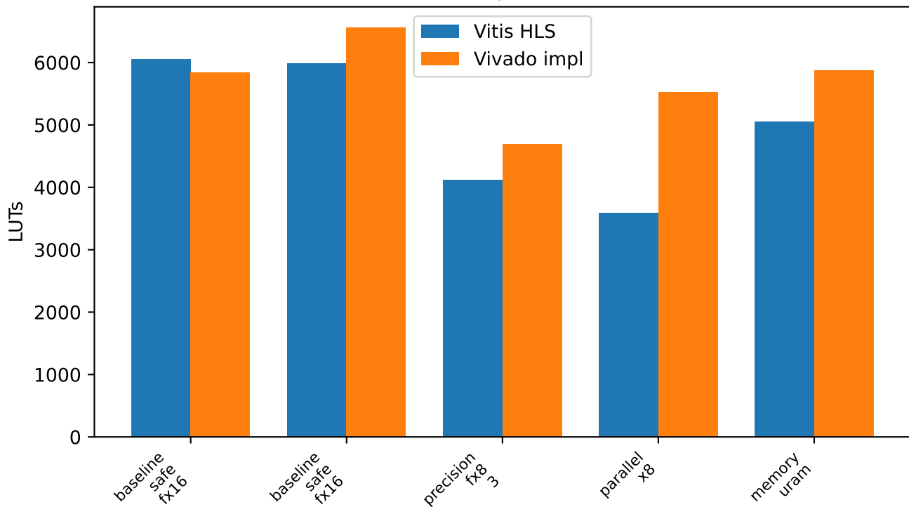
HLS vs Vivado implementation LUTs
