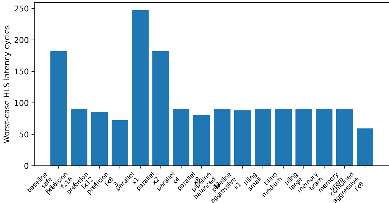
KV260 inference design knob latency effect
