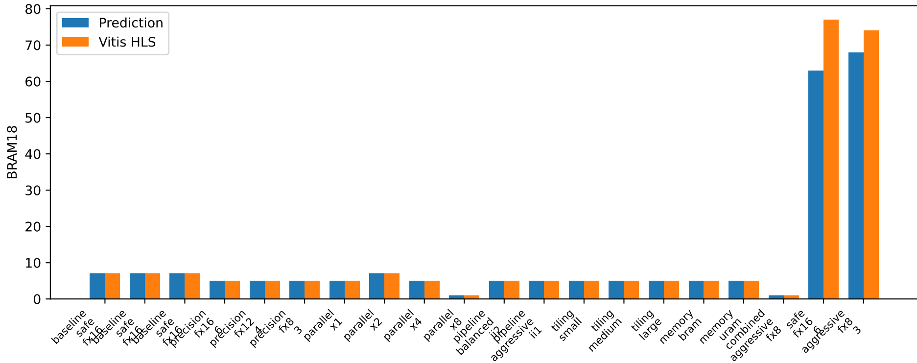
Prediction vs Vitis HLS BRAM18
