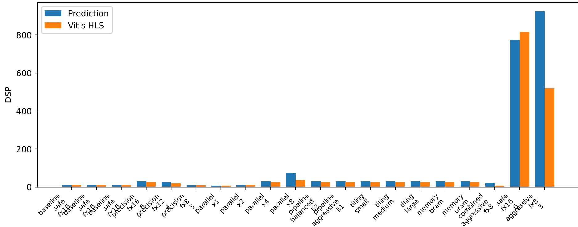
Prediction vs Vitis HLS DSP
