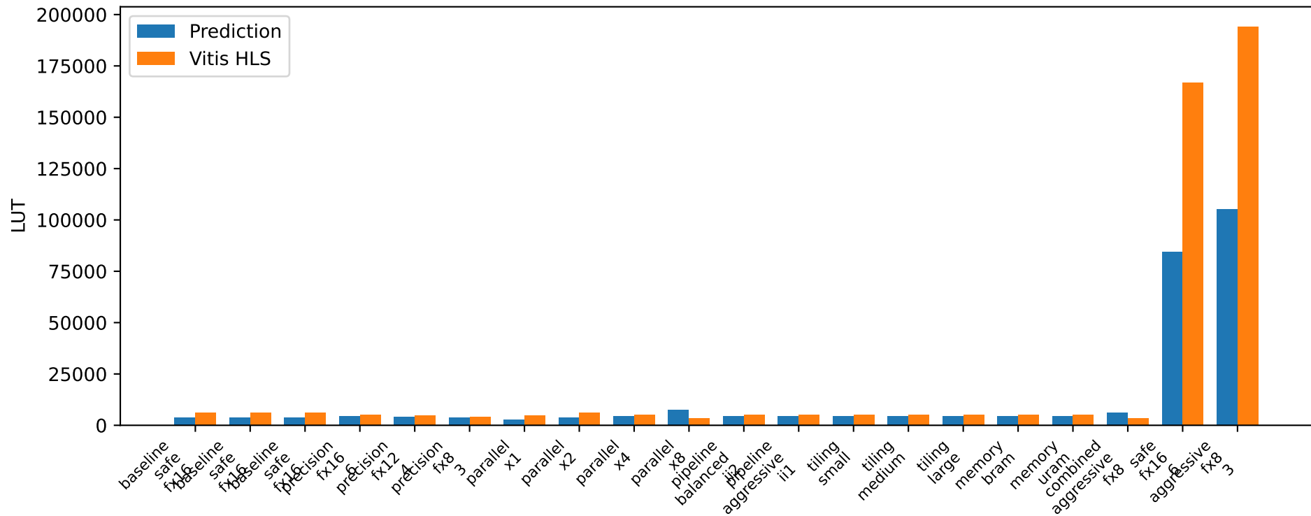
Prediction vs Vitis HLS LUT
