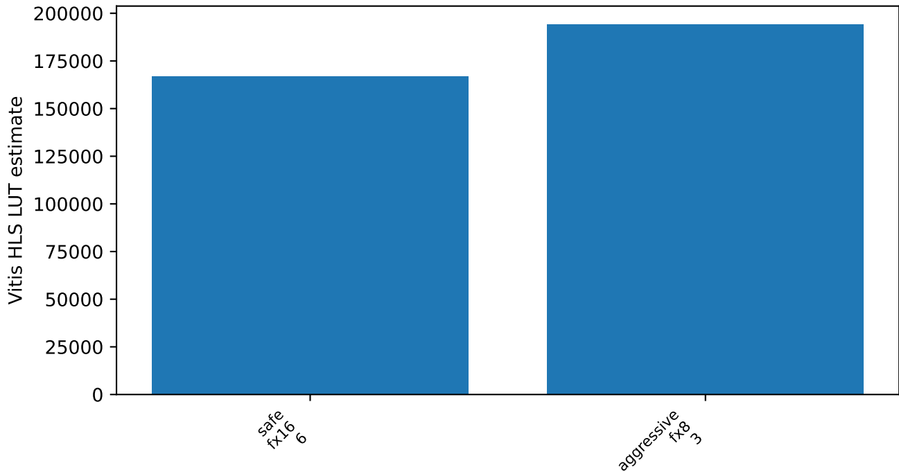
Training designs and KV260 capacity pressure
