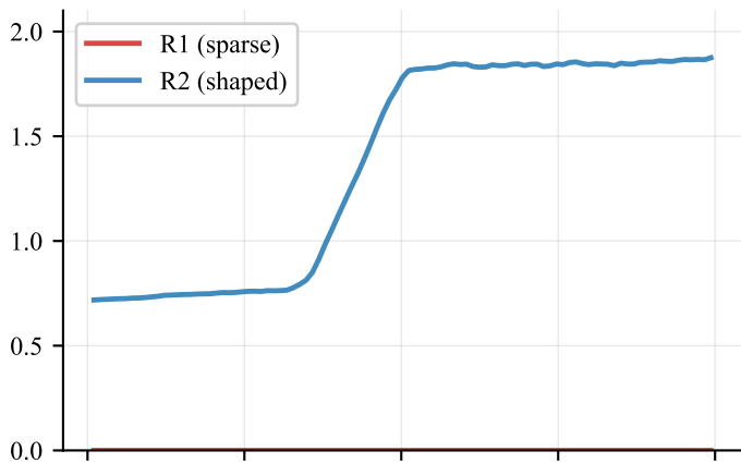
(c) Mean Episode Length
