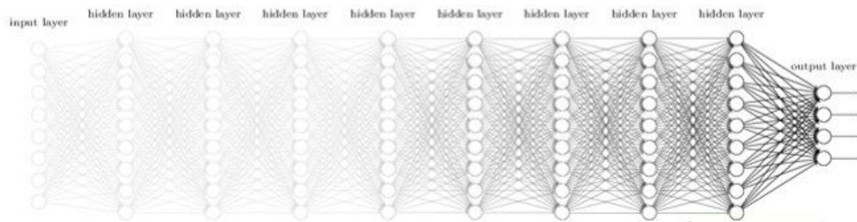
Vanishing Gradient
