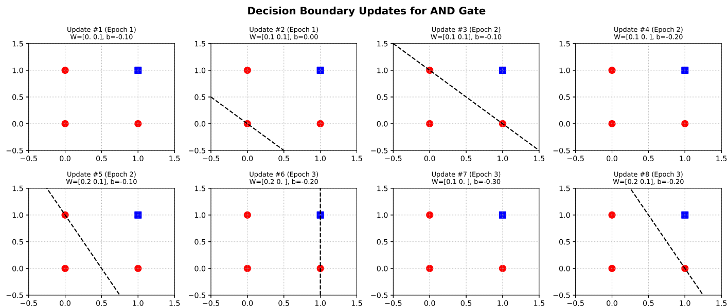
Figure 10: Decision Boundary Updates for AND gate
