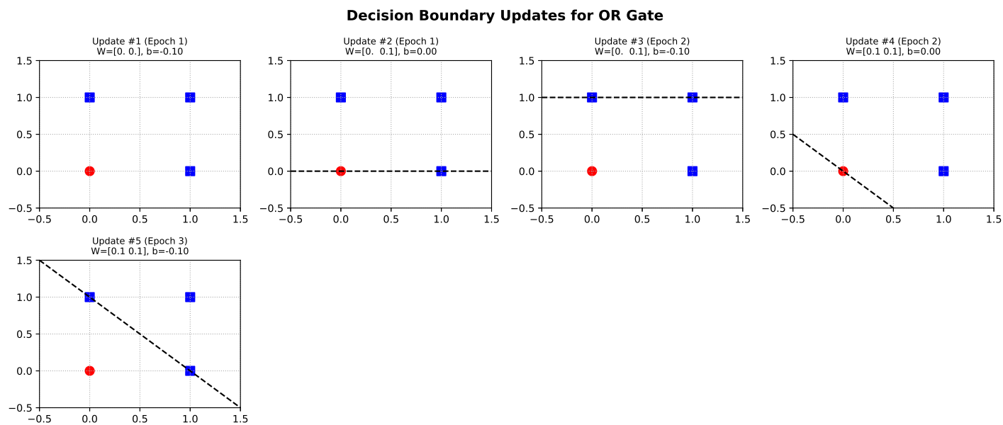
Figure 11: Decision Boundary Updates for OR gate
