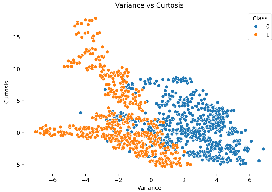
Figure 4: Variance vs Kurtosis
