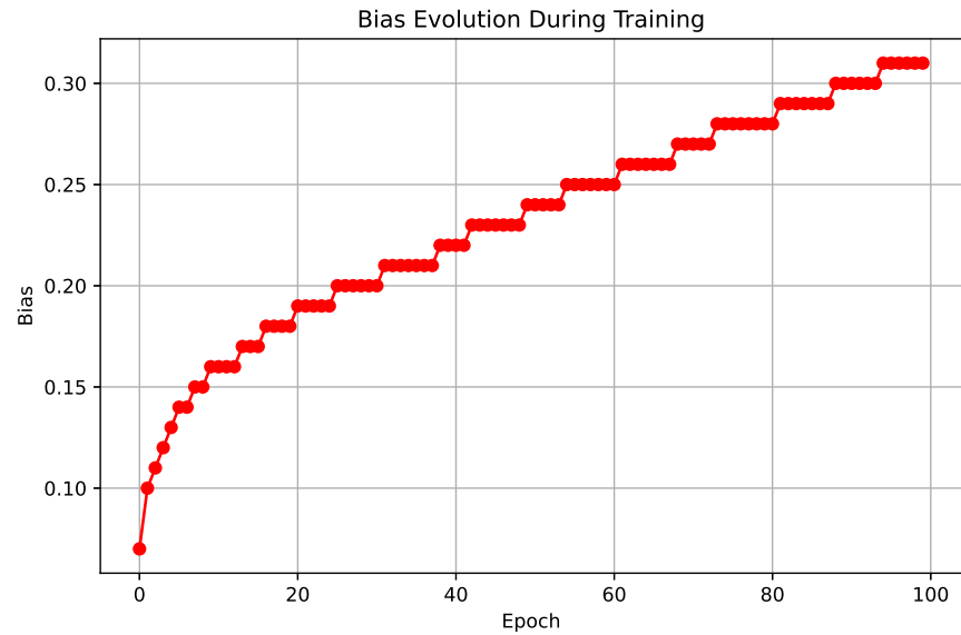
Figure 11: Bias Evolution
