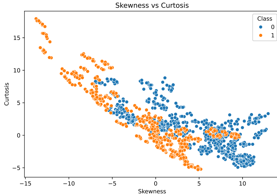
Figure 6: Skewness vs Kurtosis
