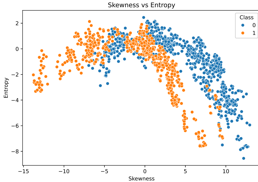
Figure 7: Skewness vs Entropy
