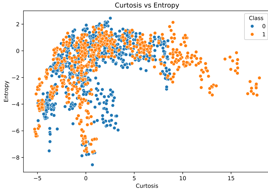
Figure 8: Curtosis vs Entropy
