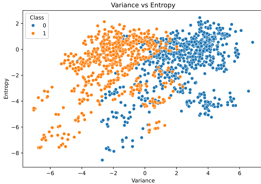
Figure 5: Variance vs Entropy
