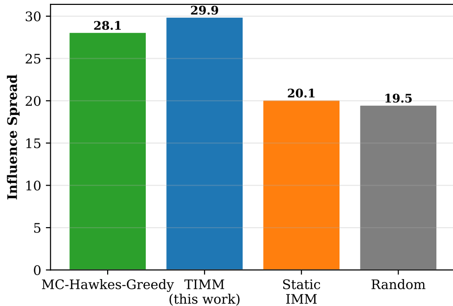
Seed Quality (Synth-S, k=10)
