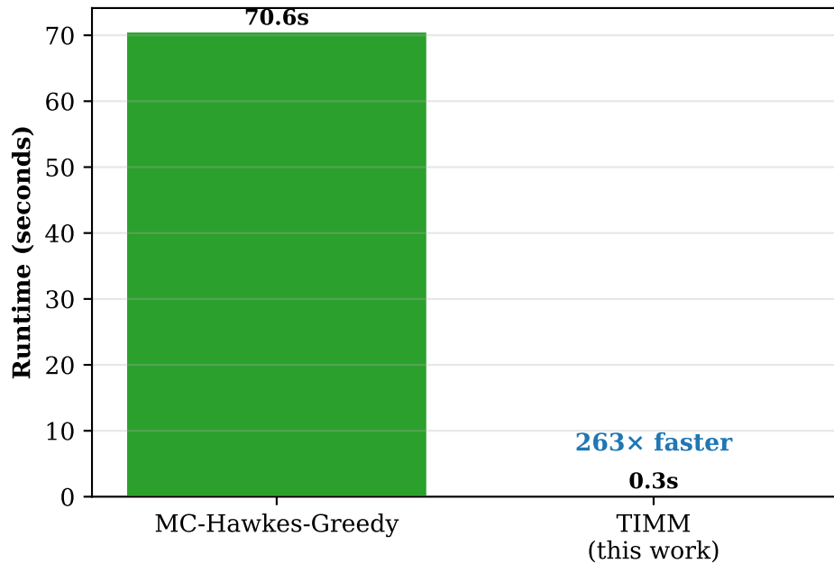
Computational Cost (Synth-S, k=10)
