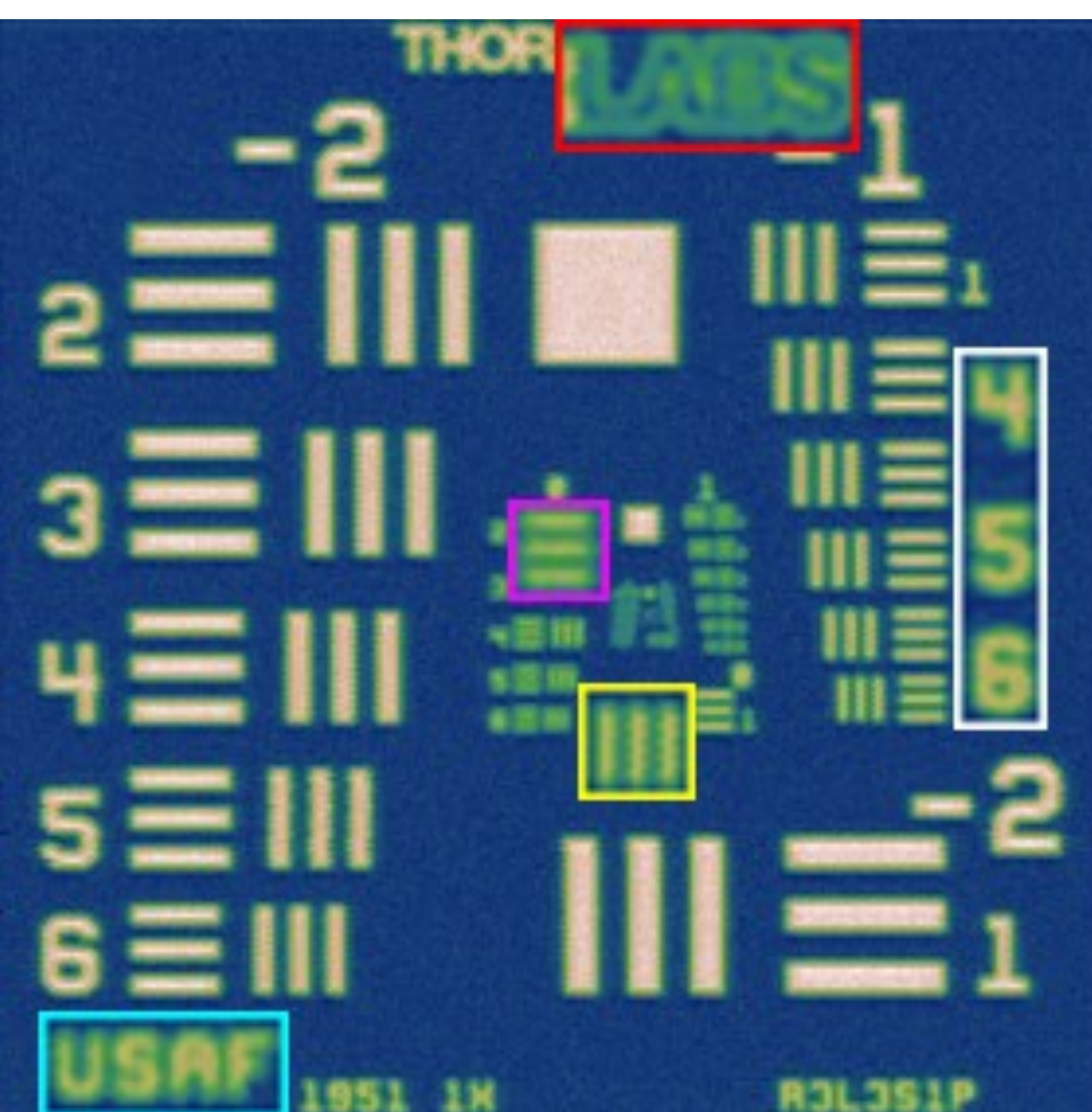
(e) I_{2.0}
