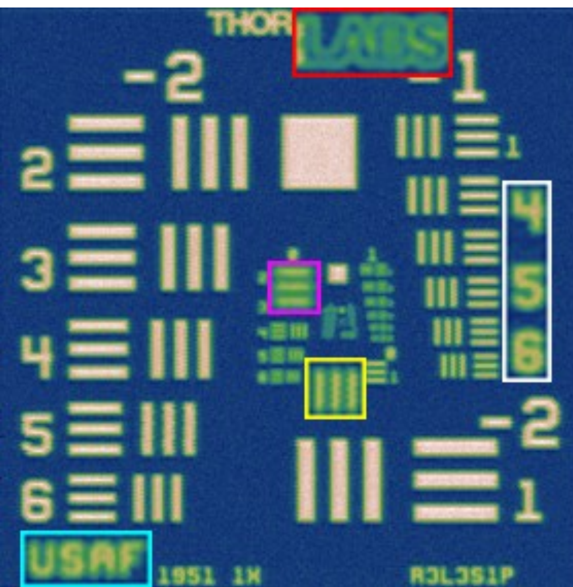
(e) I_{2.0} 15.4 / 64.76
