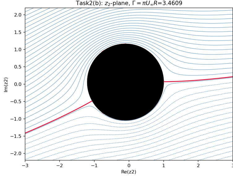
Figure 3: z_2 -plane flow with the arbitrary circulation \Gamma = \pi U_\infty R . The rear stagnation point misses the sharp corner.
