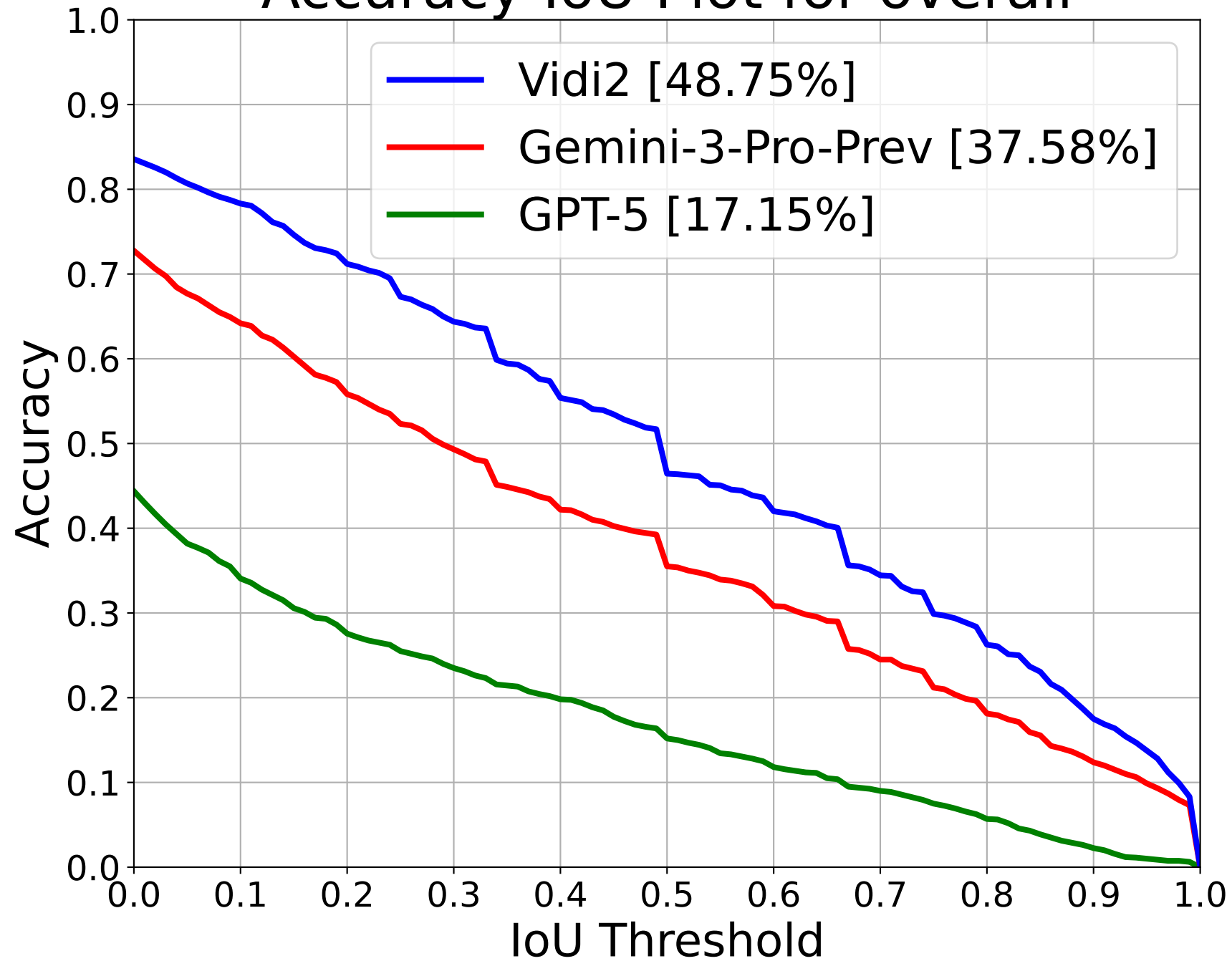
Accuracy-IoU Plot for overall
