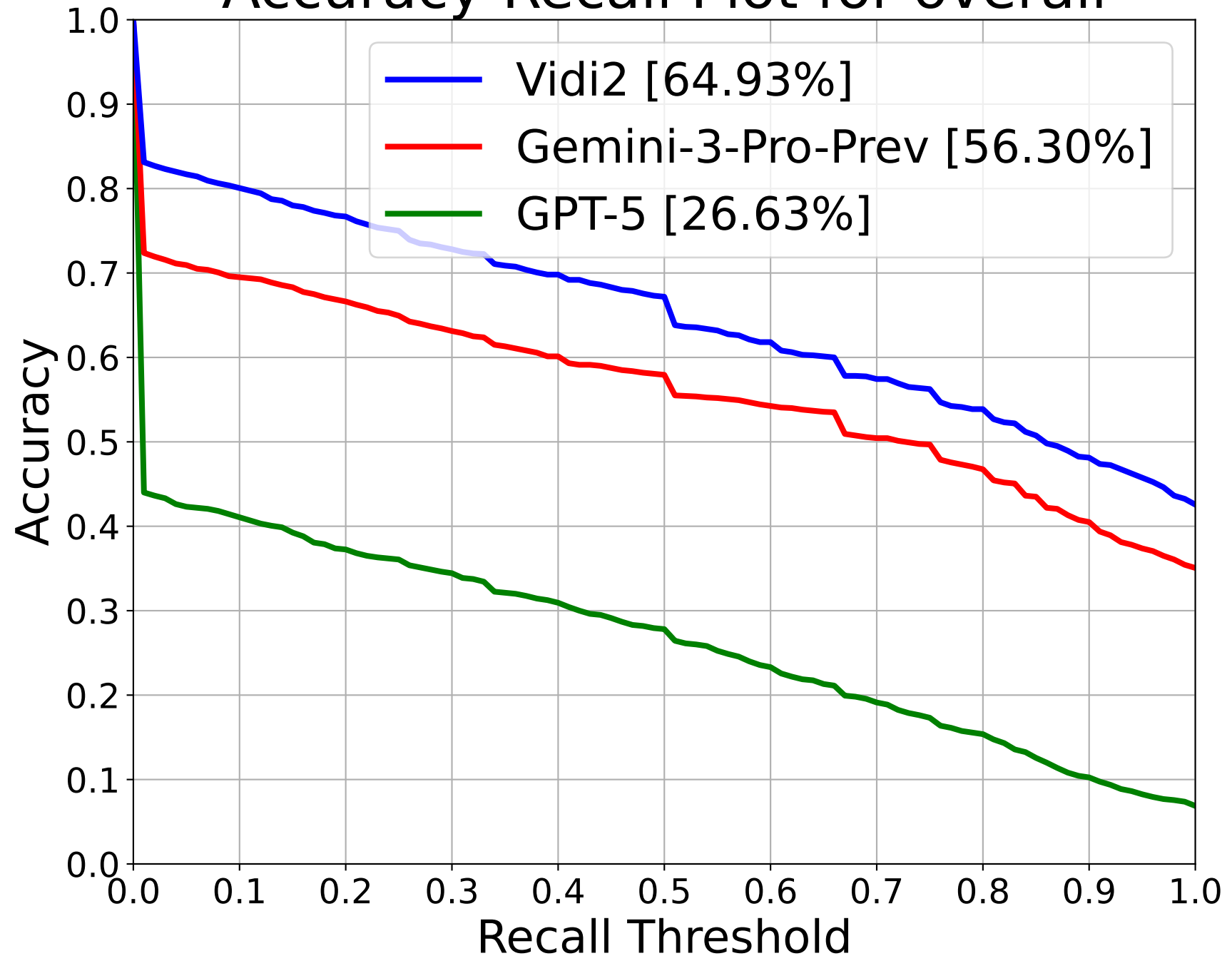
Accuracy-Recall Plot for overall
