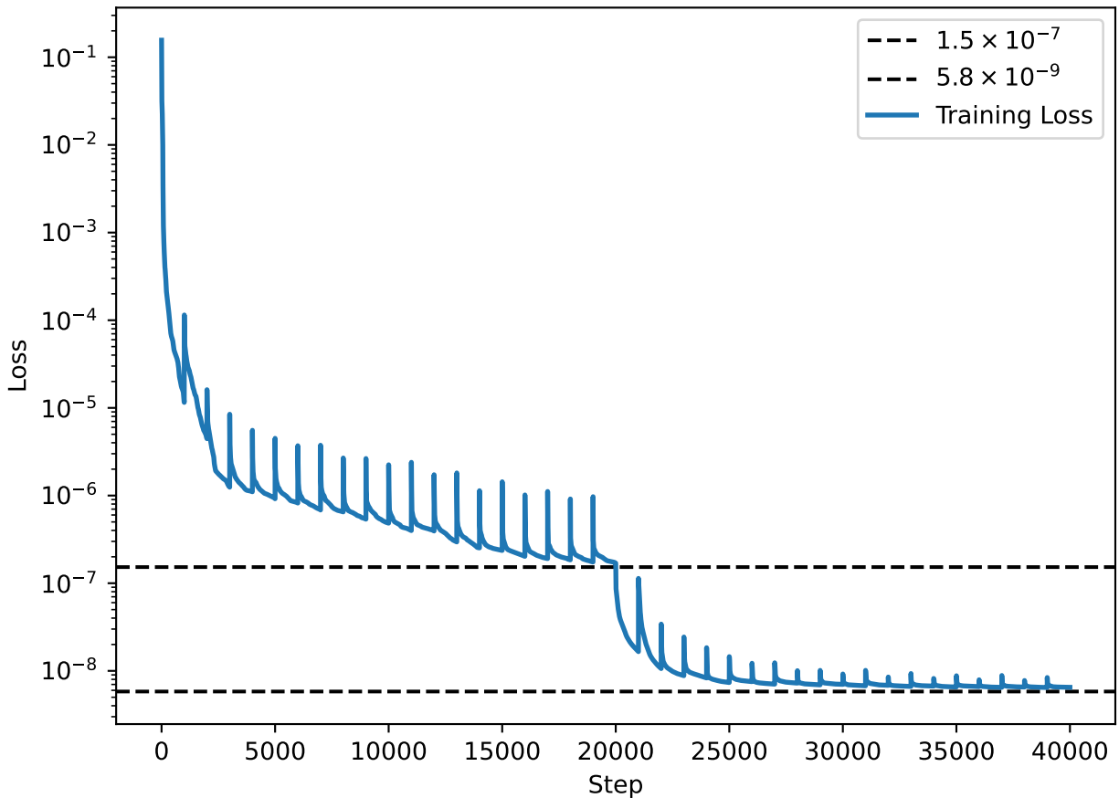
Loss, sample size 15k, model size medium
