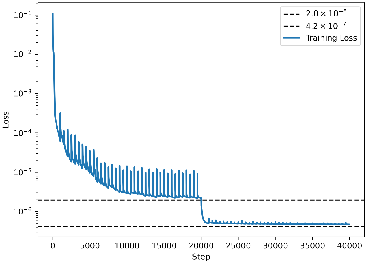
Loss, sample size 10k, model size small
