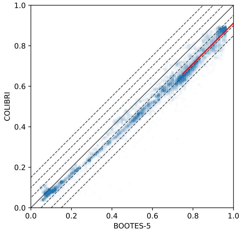
Figure 3: The differences in humidity measurements from the BOOTES-5 and COLIBRÍ stations in the second half of 2025 August and most of 2025 September. The red line shows the median offset of -9\% between humidities of 75\% and 100\% . Notice that neither station ever reads 100\% in this period, despite observed episodes of fog and rain.
